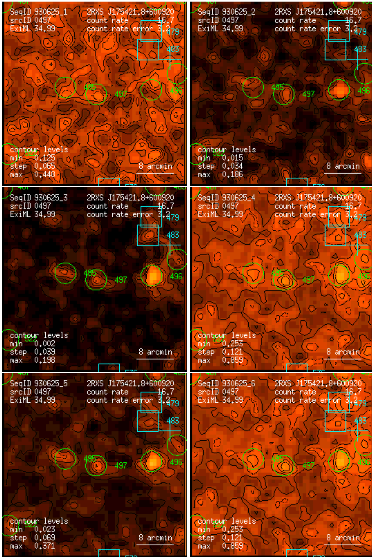
Figure 497: RASS 930625: detection 0497: band rate images, Gaussian filter: (1) PSPC channels 11 – 41, (2) 52 – 90, (3) 91 – 201, (4) 11 – 235, (5) 52 – 201, (6) 11 – 201. Broad band rates in counts/ks. Band rate contour levels in counts/ks/arcmin 2 .
