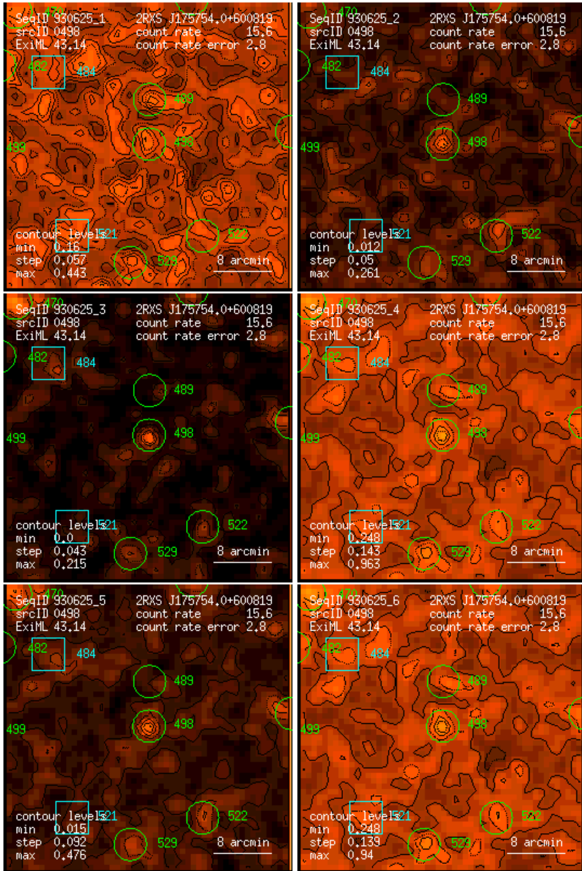
Figure 498: RASS 930625: detection 0498: band rate images, Gaussian filter: (1) PSPC channels 11 – 41, (2) 52 – 90, (3) 91 – 201, (4) 11 – 235, (5) 52 – 201, (6) 11 – 201. Broad band rates in counts/ks. Band rate contour levels in counts/ks/arcmin 2 .
