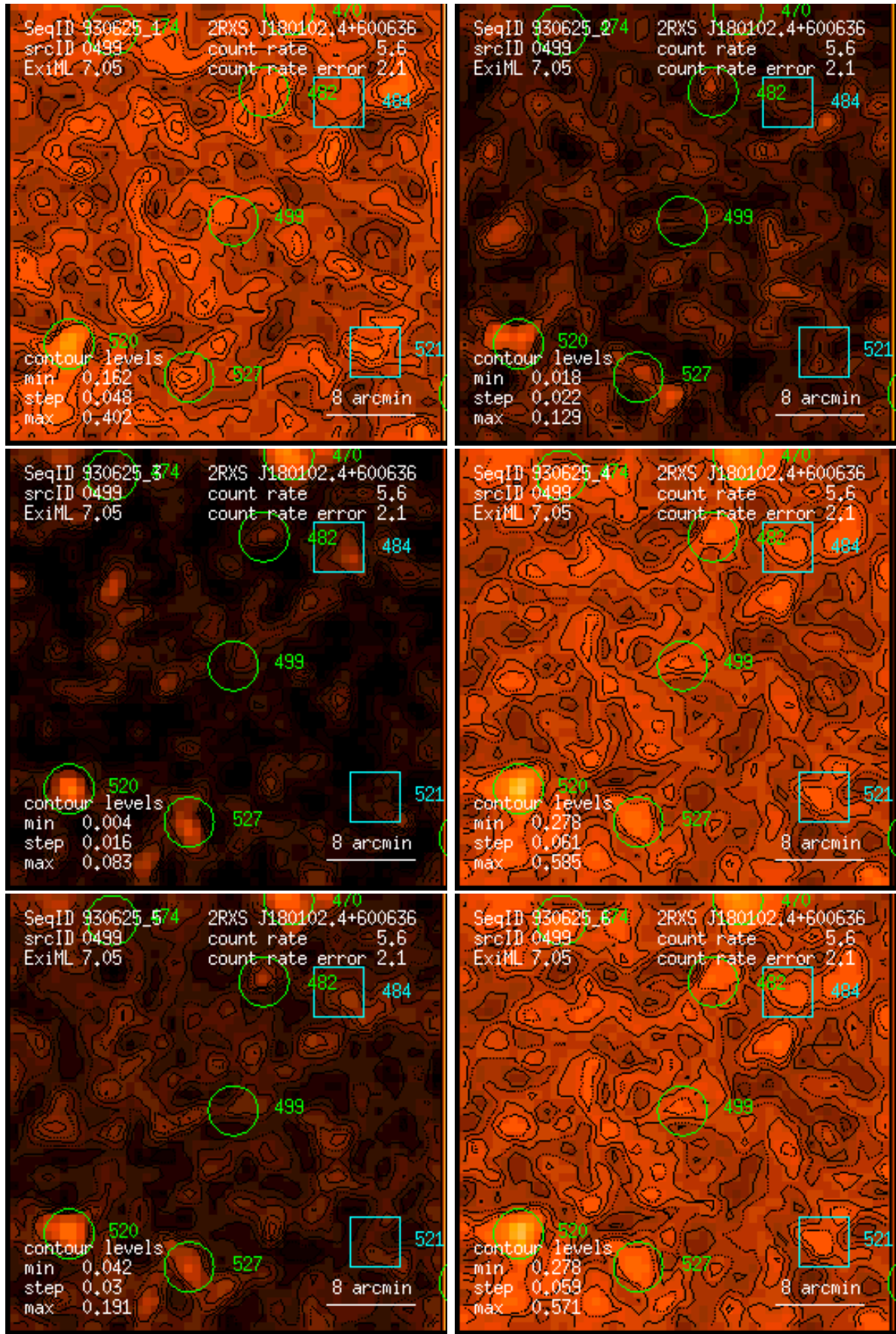
Figure 499: RASS 930625: detection 0499: band rate images, Gaussian filter: (1) PSPC channels 11 – 41, (2) 52 – 90, (3) 91 – 201, (4) 11 – 235, (5) 52 – 201, (6) 11 – 201. Broad band rates in counts/ks. Band rate contour levels in counts/ks/arcmin 2 .
