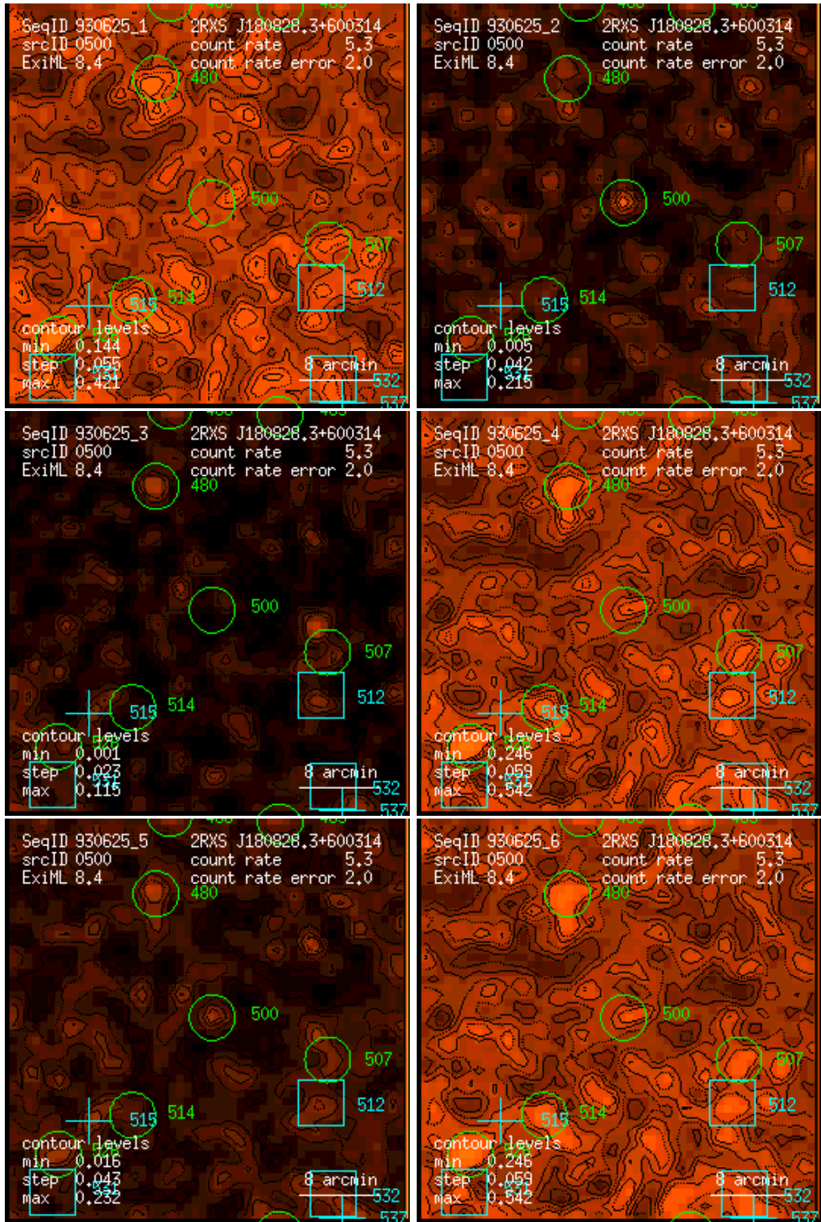
Figure 500: RASS 930625: detection 0500: band rate images, Gaussian filter: (1) PSPC channels 11 – 41, (2) 52 – 90, (3) 91 – 201, (4) 11 – 235, (5) 52 – 201, (6) 11 – 201. Broad band rates in counts/ks. Band rate contour levels in counts/ks/arcmin 2 .
