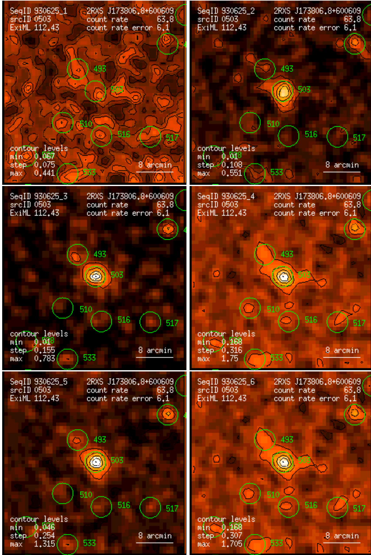
Figure 503: RASS 930625: detection 0503: band rate images, Gaussian filter: (1) PSPC channels 11 – 41, (2) 52 – 90, (3) 91 – 201, (4) 11 – 235, (5) 52 – 201, (6) 11 – 201. Broad band rates in counts/ks. Band rate contour levels in counts/ks/arcmin 2 .
