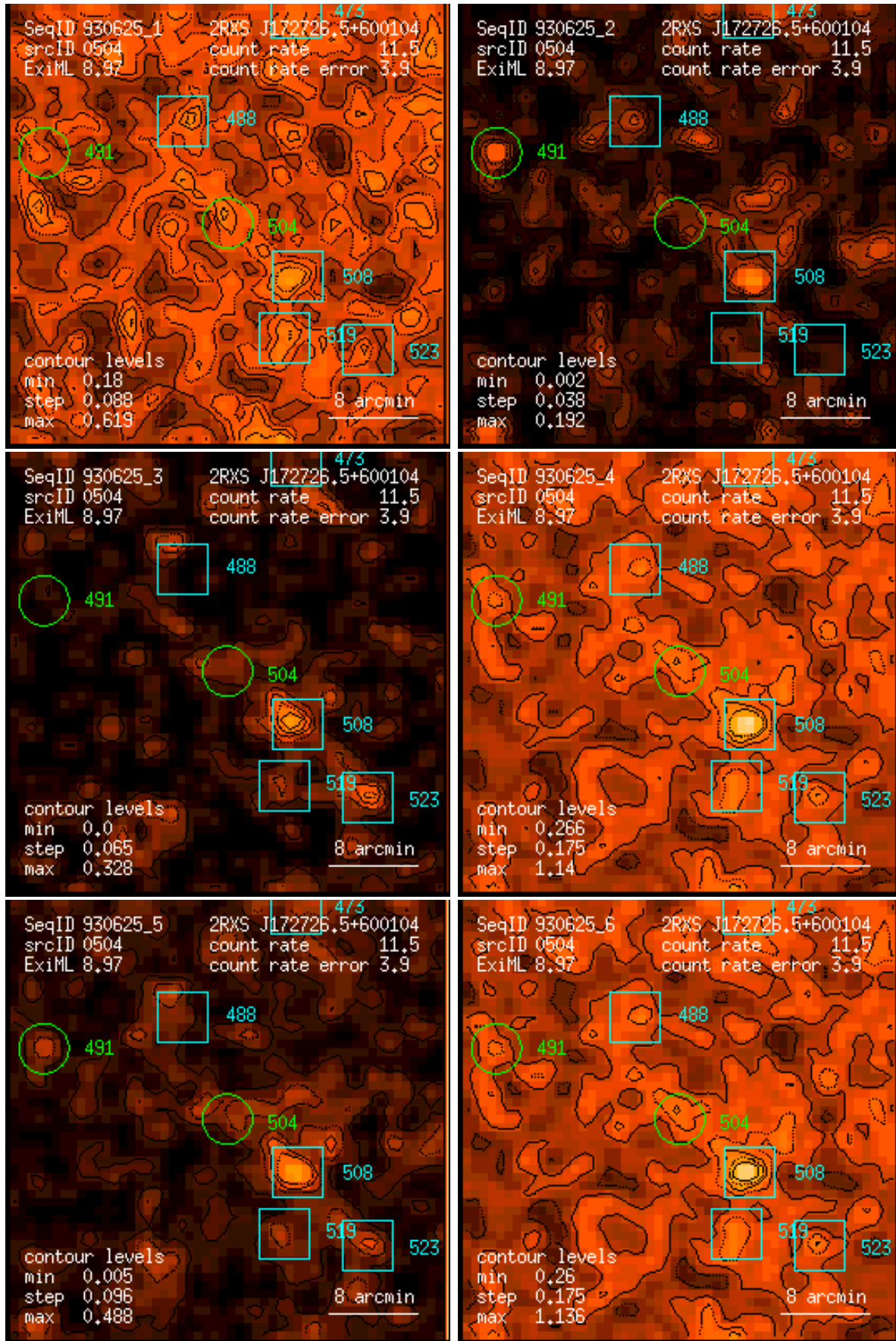
Figure 504: RASS 930625: detection 0504: band rate images, Gaussian filter: (1) PSPC channels 11 – 41, (2) 52 – 90, (3) 91 – 201, (4) 11 – 235, (5) 52 – 201, (6) 11 – 201. Broad band rates in counts/ks. Band rate contour levels in counts/ks/arcmin 2 .
