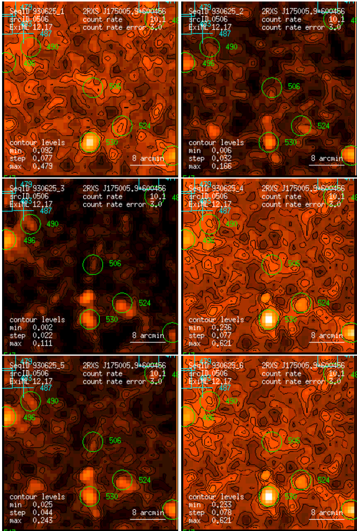
Figure 506: RASS 930625: detection 0506: band rate images, Gaussian filter: (1) PSPC channels 11 – 41, (2) 52 – 90, (3) 91 – 201, (4) 11 – 235, (5) 52 – 201, (6) 11 – 201. Broad band rates in counts/ks. Band rate contour levels in counts/ks/arcmin 2 .
