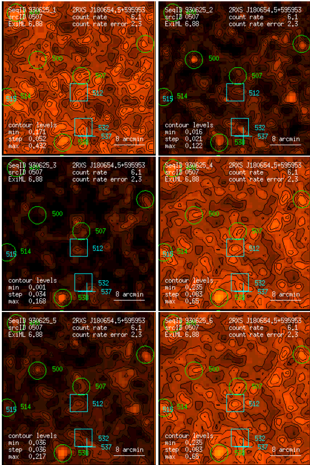
Figure 507: RASS 930625: detection 0507: band rate images, Gaussian filter: (1) PSPC channels 11 – 41, (2) 52 – 90, (3) 91 – 201, (4) 11 – 235, (5) 52 – 201, (6) 11 – 201. Broad band rates in counts/ks. Band rate contour levels in counts/ks/arcmin 2 .
