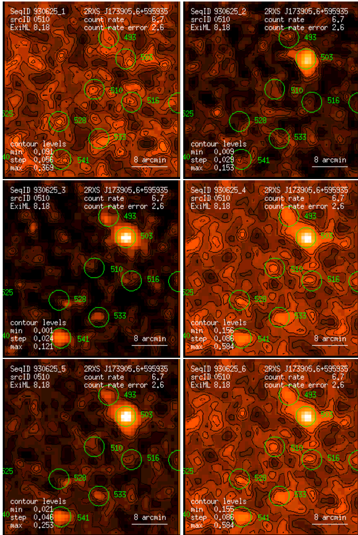
Figure 510: RASS 930625: detection 0510: band rate images, Gaussian filter: (1) PSPC channels 11 – 41, (2) 52 – 90, (3) 91 – 201, (4) 11 – 235, (5) 52 – 201, (6) 11 – 201. Broad band rates in counts/ks. Band rate contour levels in counts/ks/arcmin 2 .
