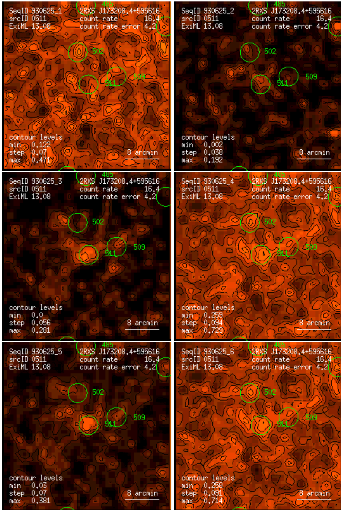
Figure 511: RASS 930625: detection 0511: band rate images, Gaussian filter: (1) PSPC channels 11 – 41, (2) 52 – 90, (3) 91 – 201, (4) 11 – 235, (5) 52 – 201, (6) 11 – 201. Broad band rates in counts/ks. Band rate contour levels in counts/ks/arcmin 2 .
