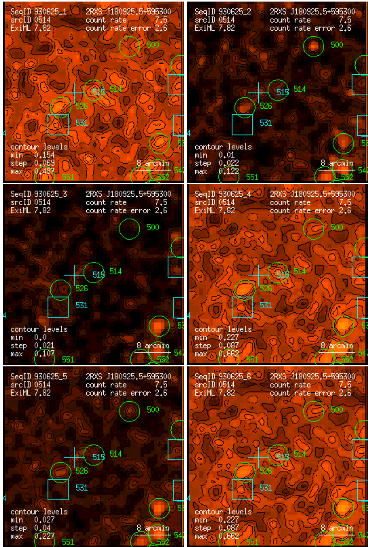
Figure 514: RASS 930625: detection 0514: band rate images, Gaussian filter: (1) PSPC channels 11 – 41, (2) 52 – 90, (3) 91 – 201, (4) 11 – 235, (5) 52 – 201, (6) 11 – 201. Broad band rates in counts/ks. Band rate contour levels in counts/ks/arcmin 2 .
