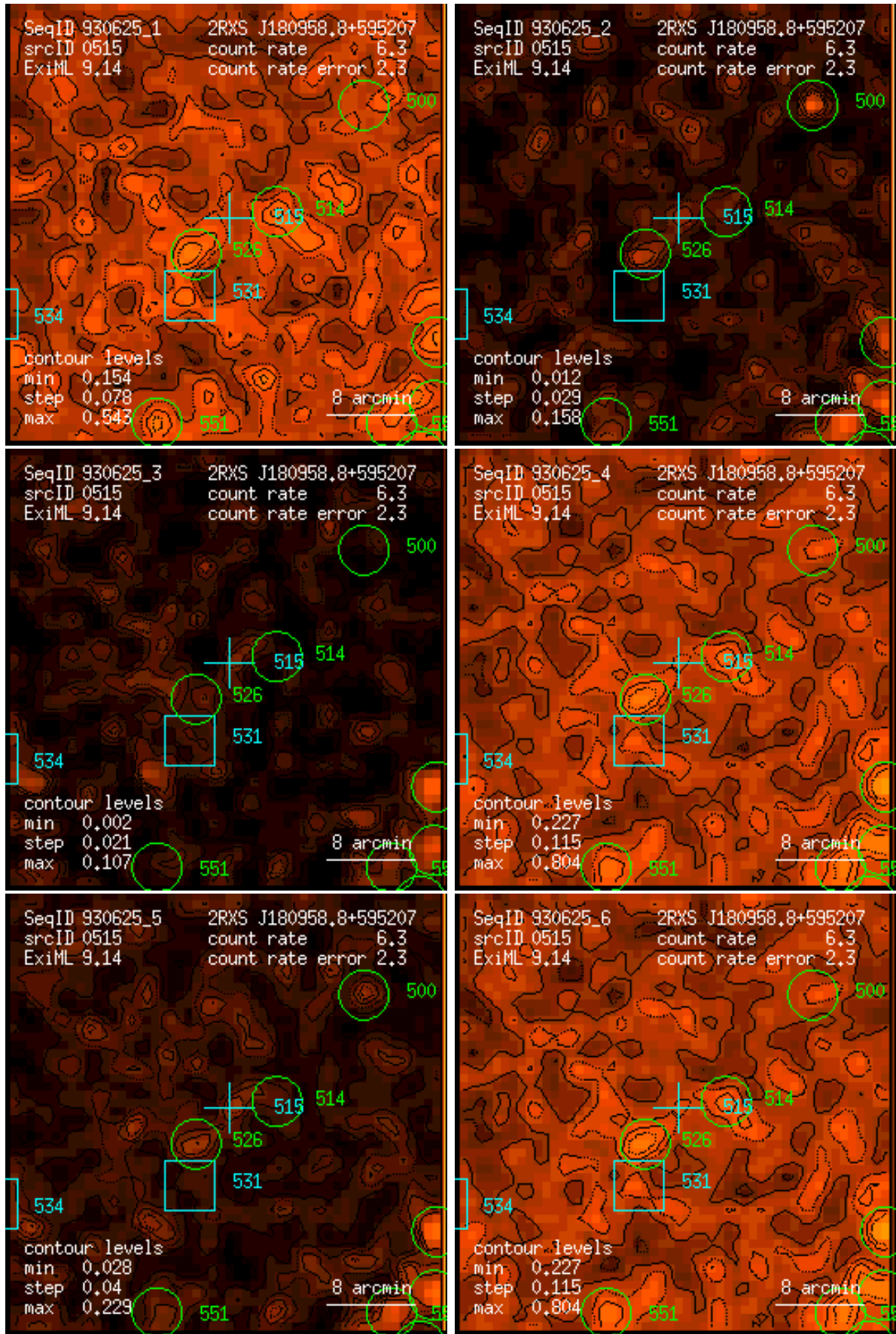
Figure 515: RASS 930625: detection 0515: band rate images, Gaussian filter: (1) PSPC channels 11 – 41, (2) 52 – 90, (3) 91 – 201, (4) 11 – 235, (5) 52 – 201, (6) 11 – 201. Broad band rates in counts/ks. Band rate contour levels in counts/ks/arcmin 2 .
