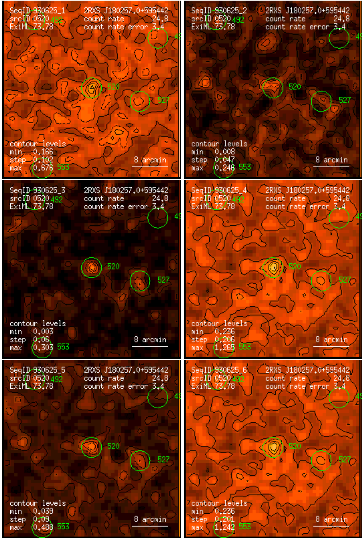
Figure 520: RASS 930625: detection 0520: band rate images, Gaussian filter: (1) PSPC channels 11 – 41, (2) 52 – 90, (3) 91 – 201, (4) 11 – 235, (5) 52 – 201, (6) 11 – 201. Broad band rates in counts/ks. Band rate contour levels in counts/ks/arcmin 2 .
