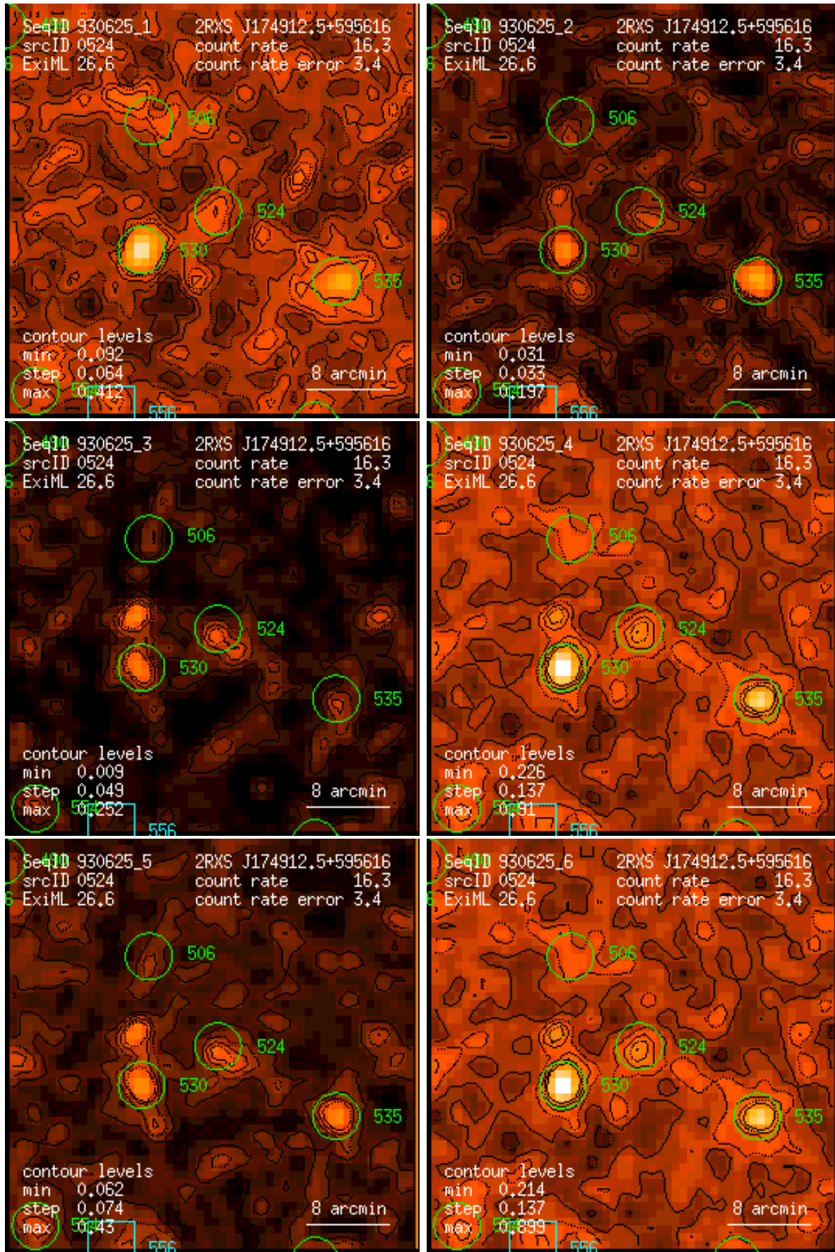
Figure 524: RASS 930625: detection 0524: band rate images, Gaussian filter: (1) PSPC channels 11 – 41, (2) 52 – 90, (3) 91 – 201, (4) 11 – 235, (5) 52 – 201, (6) 11 – 201. Broad band rates in counts/ks. Band rate contour levels in counts/ks/arcmin 2 .
