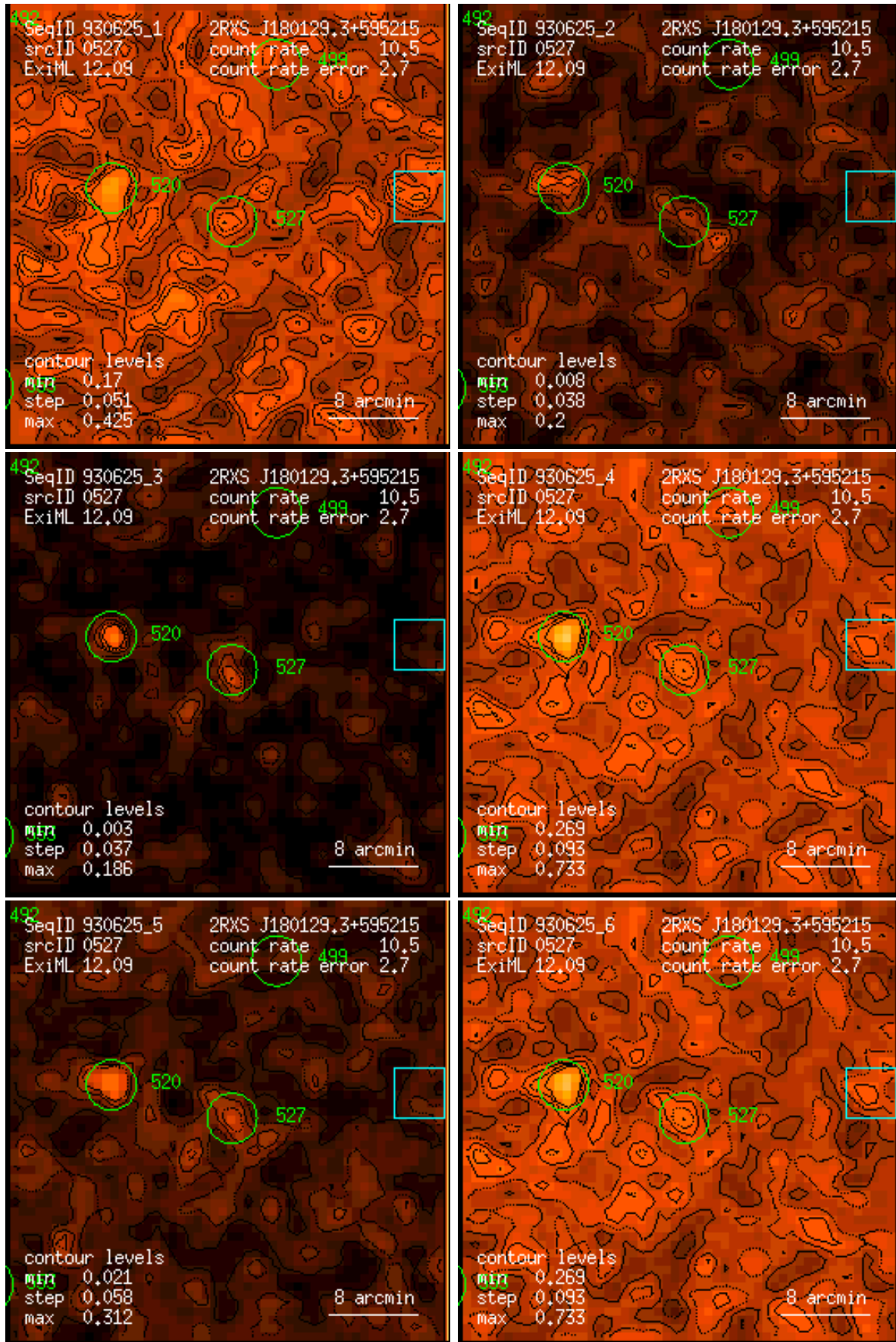
Figure 527: RASS 930625: detection 0527: band rate images, Gaussian filter: (1) PSPC channels 11 – 41, (2) 52 – 90, (3) 91 – 201, (4) 11 – 235, (5) 52 – 201, (6) 11 – 201. Broad band rates in counts/ks. Band rate contour levels in counts/ks/arcmin 2 .
