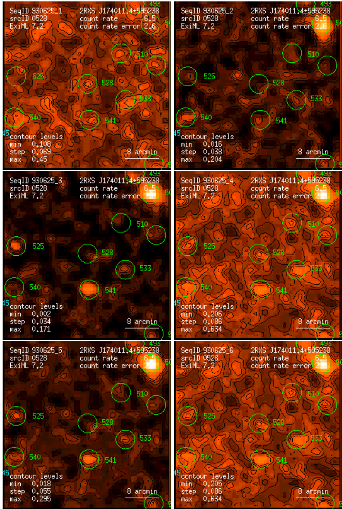
Figure 528: RASS 930625: detection 0528: band rate images, Gaussian filter: (1) PSPC channels 11 – 41, (2) 52 – 90, (3) 91 – 201, (4) 11 – 235, (5) 52 – 201, (6) 11 – 201. Broad band rates in counts/ks. Band rate contour levels in counts/ks/arcmin 2 .
