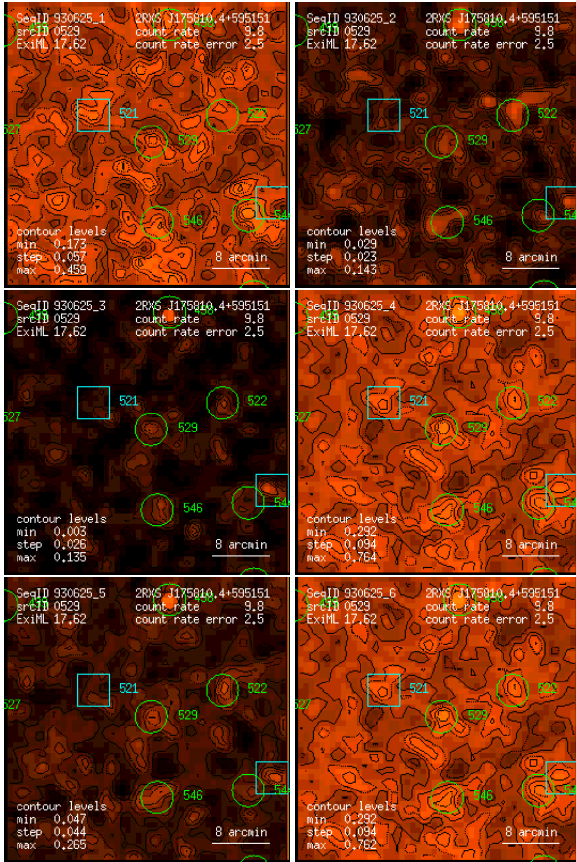
Figure 529: RASS 930625: detection 0529: band rate images, Gaussian filter: (1) PSPC channels 11 – 41, (2) 52 – 90, (3) 91 – 201, (4) 11 – 235, (5) 52 – 201, (6) 11 – 201. Broad band rates in counts/ks. Band rate contour levels in counts/ks/arcmin 2 .
