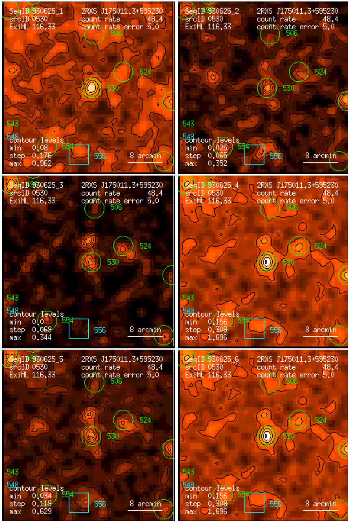
Figure 530: RASS 930625: detection 0530: band rate images, Gaussian filter: (1) PSPC channels 11 – 41, (2) 52 – 90, (3) 91 – 201, (4) 11 – 235, (5) 52 – 201, (6) 11 – 201. Broad band rates in counts/ks. Band rate contour levels in counts/ks/arcmin 2 .
