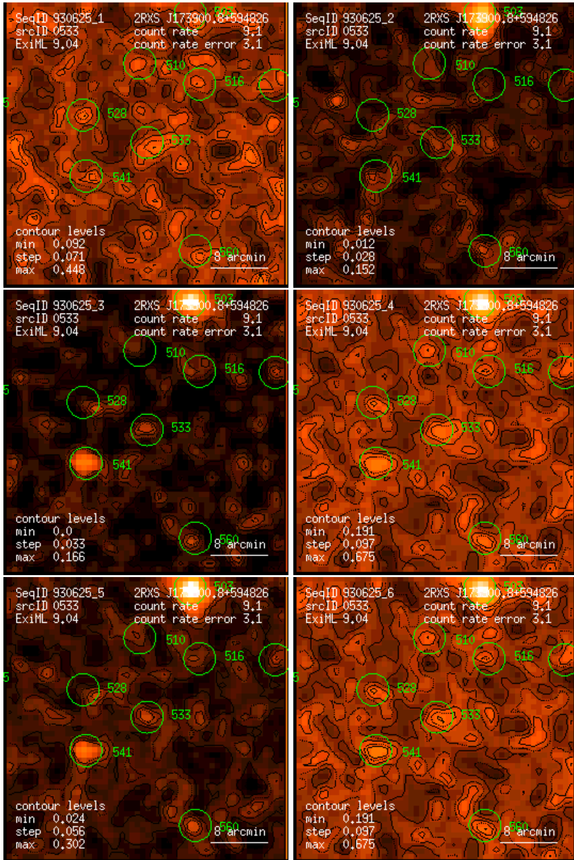
Figure 533: RASS 930625: detection 0533: band rate images, Gaussian filter: (1) PSPC channels 11 – 41, (2) 52 – 90, (3) 91 – 201, (4) 11 – 235, (5) 52 – 201, (6) 11 – 201. Broad band rates in counts/ks. Band rate contour levels in counts/ks/arcmin 2 .
