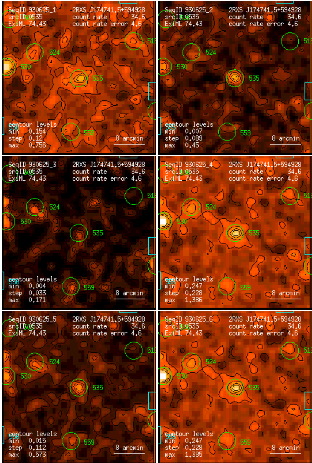
Figure 535: RASS 930625: detection 0535: band rate images, Gaussian filter: (1) PSPC channels 11 – 41, (2) 52 – 90, (3) 91 – 201, (4) 11 – 235, (5) 52 – 201, (6) 11 – 201. Broad band rates in counts/ks. Band rate contour levels in counts/ks/arcmin 2 .
