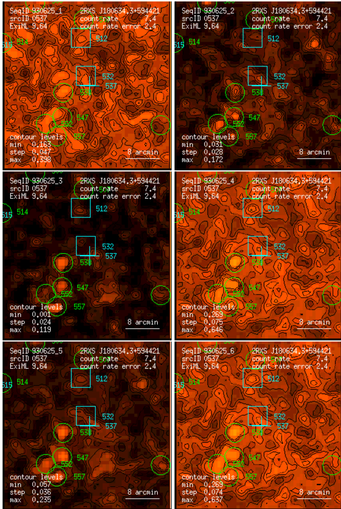
Figure 537: RASS 930625: detection 0537: band rate images, Gaussian filter: (1) PSPC channels 11 – 41, (2) 52 – 90, (3) 91 – 201, (4) 11 – 235, (5) 52 – 201, (6) 11 – 201. Broad band rates in counts/ks. Band rate contour levels in counts/ks/arcmin 2 .
