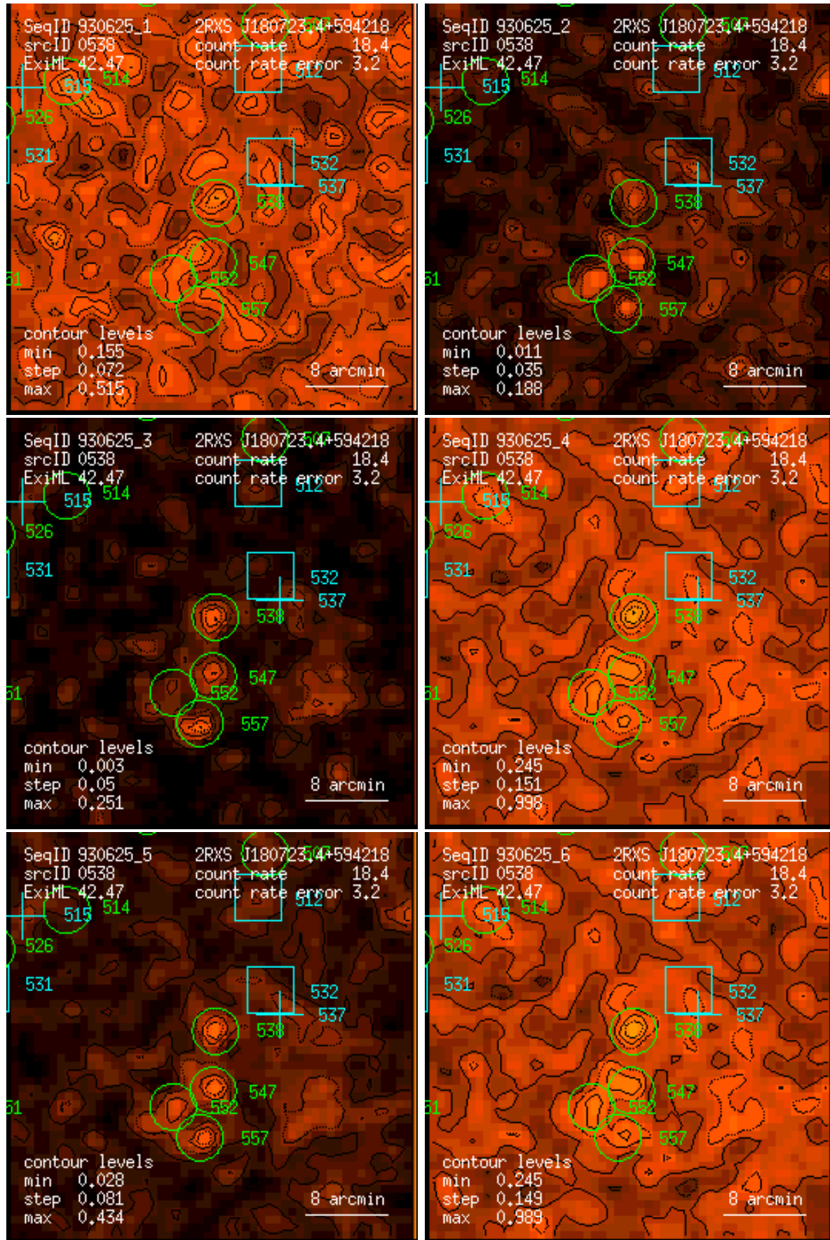
Figure 538: RASS 930625: detection 0538: band rate images, Gaussian filter: (1) PSPC channels 11 – 41, (2) 52 – 90, (3) 91 – 201, (4) 11 – 235, (5) 52 – 201, (6) 11 – 201. Broad band rates in counts/ks. Band rate contour levels in counts/ks/arcmin 2 .
