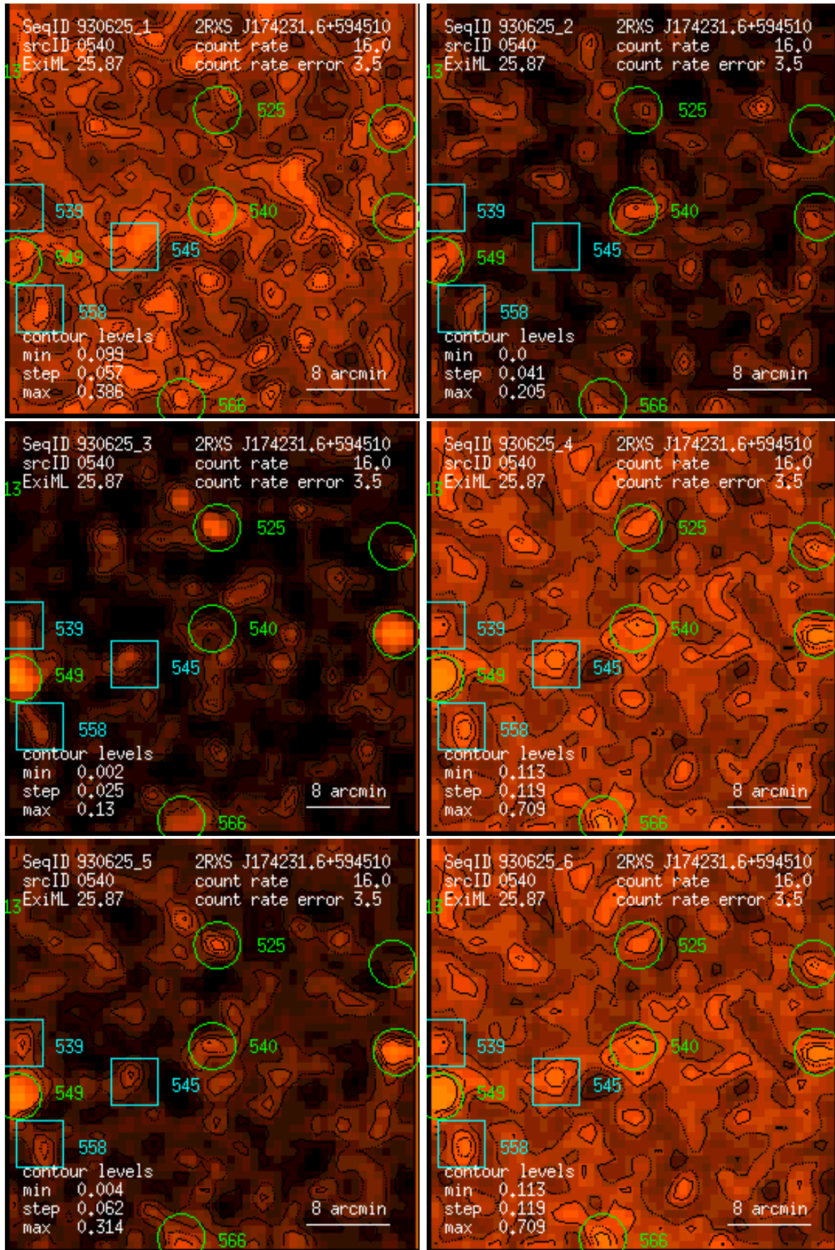
Figure 540: RASS 930625: detection 0540: band rate images, Gaussian filter: (1) PSPC channels 11 – 41, (2) 52 – 90, (3) 91 – 201, (4) 11 – 235, (5) 52 – 201, (6) 11 – 201. Broad band rates in counts/ks. Band rate contour levels in counts/ks/arcmin 2 .
