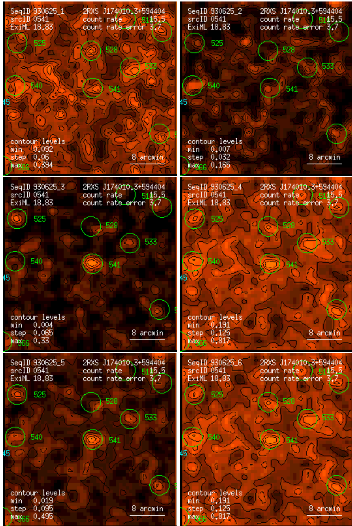
Figure 541: RASS 930625: detection 0541: band rate images, Gaussian filter: (1) PSPC channels 11 – 41, (2) 52 – 90, (3) 91 – 201, (4) 11 – 235, (5) 52 – 201, (6) 11 – 201. Broad band rates in counts/ks. Band rate contour levels in counts/ks/arcmin 2 .
