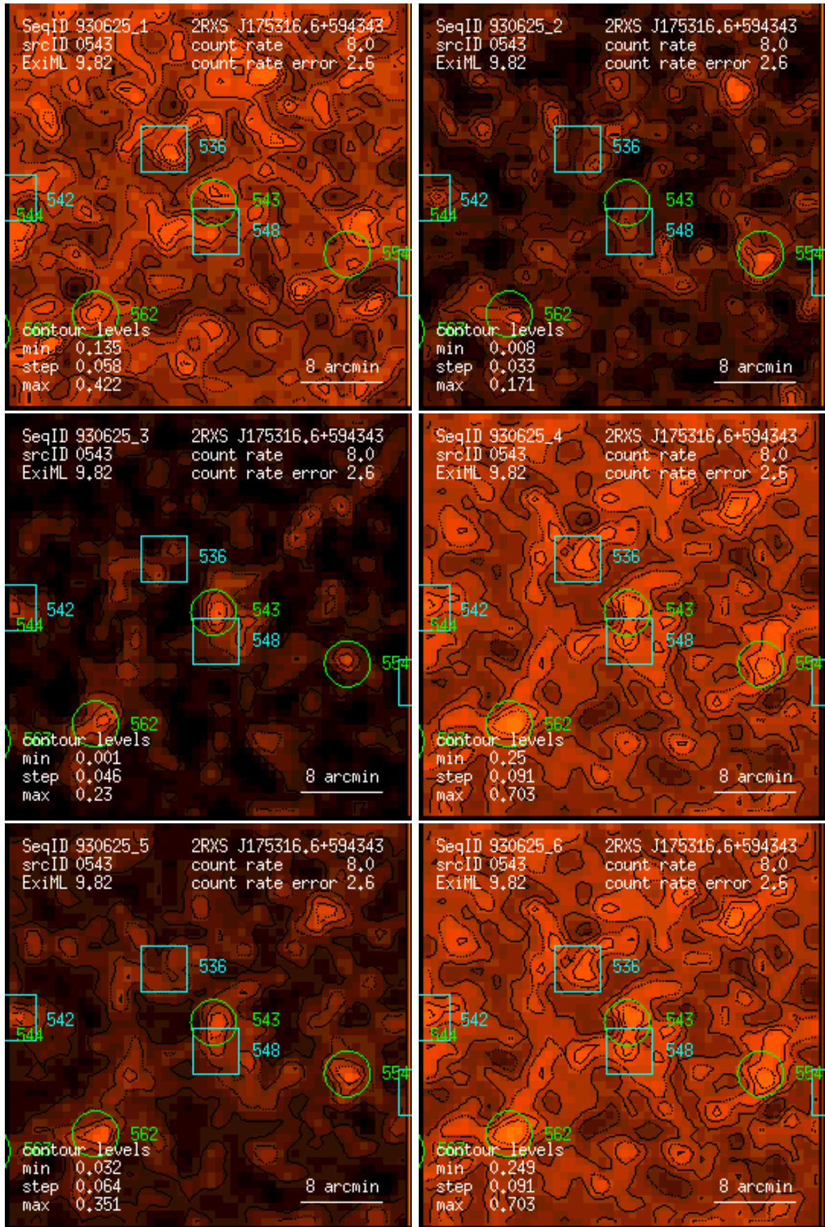
Figure 543: RASS 930625: detection 0543: band rate images, Gaussian filter: (1) PSPC channels 11 – 41, (2) 52 – 90, (3) 91 – 201, (4) 11 – 235, (5) 52 – 201, (6) 11 – 201. Broad band rates in counts/ks. Band rate contour levels in counts/ks/arcmin 2 .
