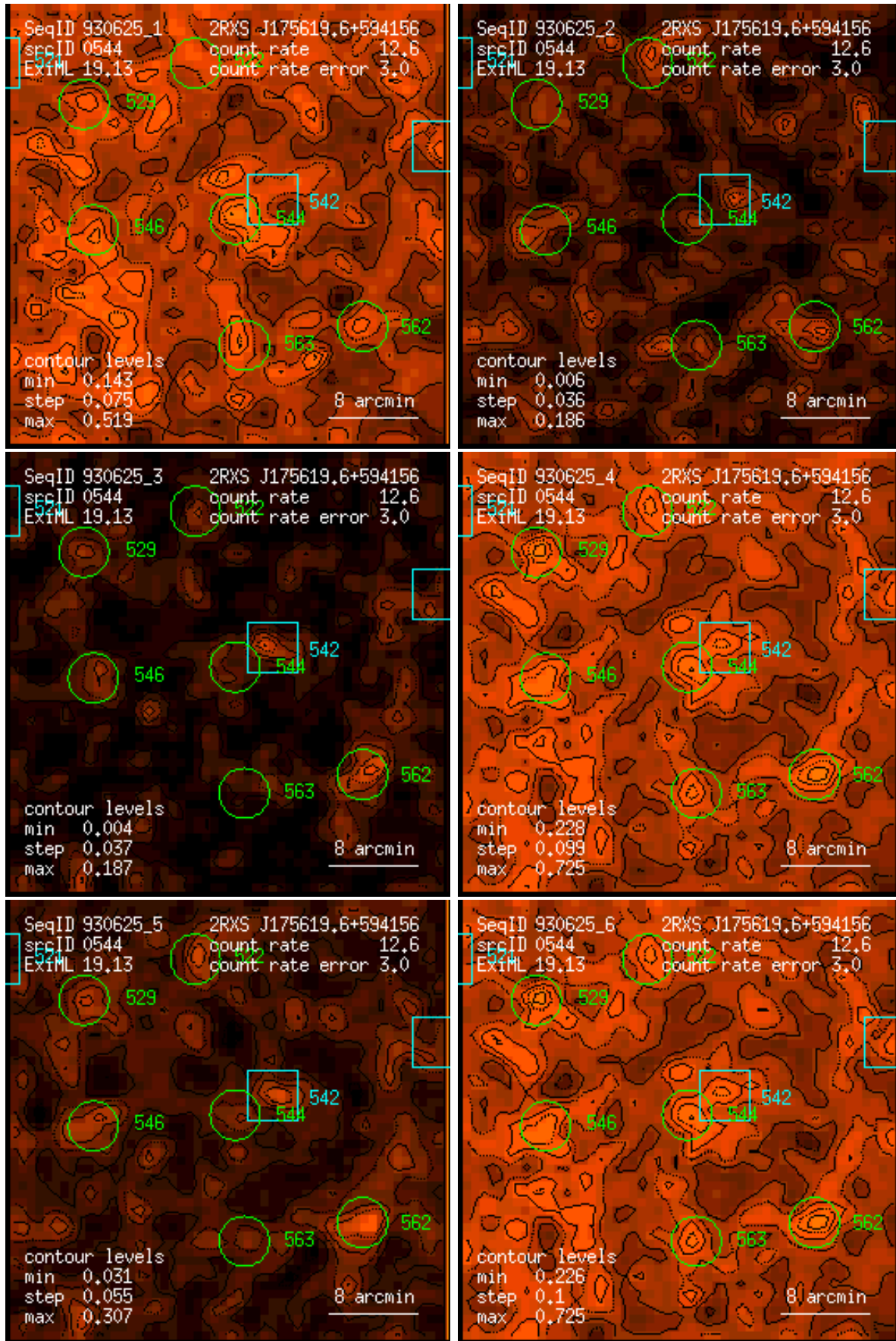
Figure 544: RASS 930625: detection 0544: band rate images, Gaussian filter: (1) PSPC channels 11 – 41, (2) 52 – 90, (3) 91 – 201, (4) 11 – 235, (5) 52 – 201, (6) 11 – 201. Broad band rates in counts/ks. Band rate contour levels in counts/ks/arcmin 2 .
