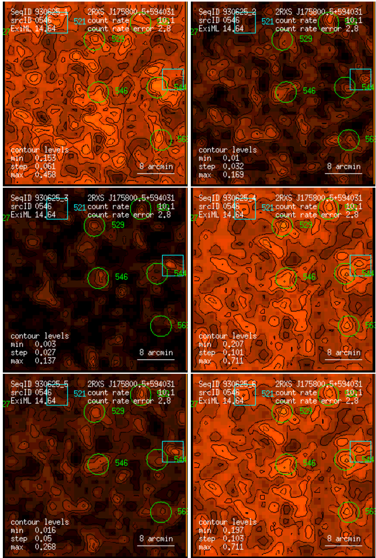
Figure 546: RASS 930625: detection 0546: band rate images, Gaussian filter: (1) PSPC channels 11 – 41, (2) 52 – 90, (3) 91 – 201, (4) 11 – 235, (5) 52 – 201, (6) 11 – 201. Broad band rates in counts/ks. Band rate contour levels in counts/ks/arcmin 2 .
