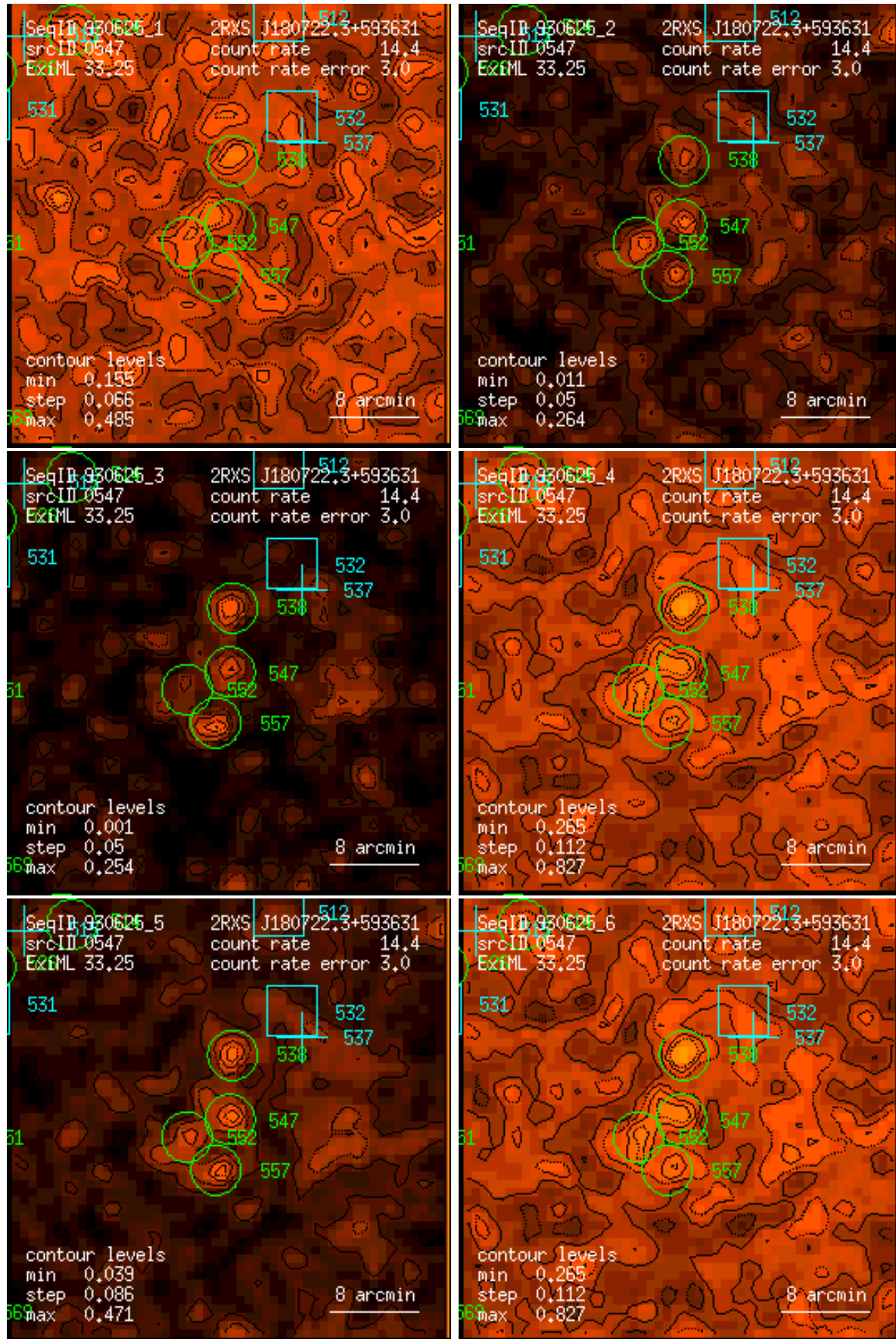
Figure 547: RASS 930625: detection 0547: band rate images, Gaussian filter: (1) PSPC channels 11 – 41, (2) 52 – 90, (3) 91 – 201, (4) 11 – 235, (5) 52 – 201, (6) 11 – 201. Broad band rates in counts/ks. Band rate contour levels in counts/ks/arcmin 2 .
