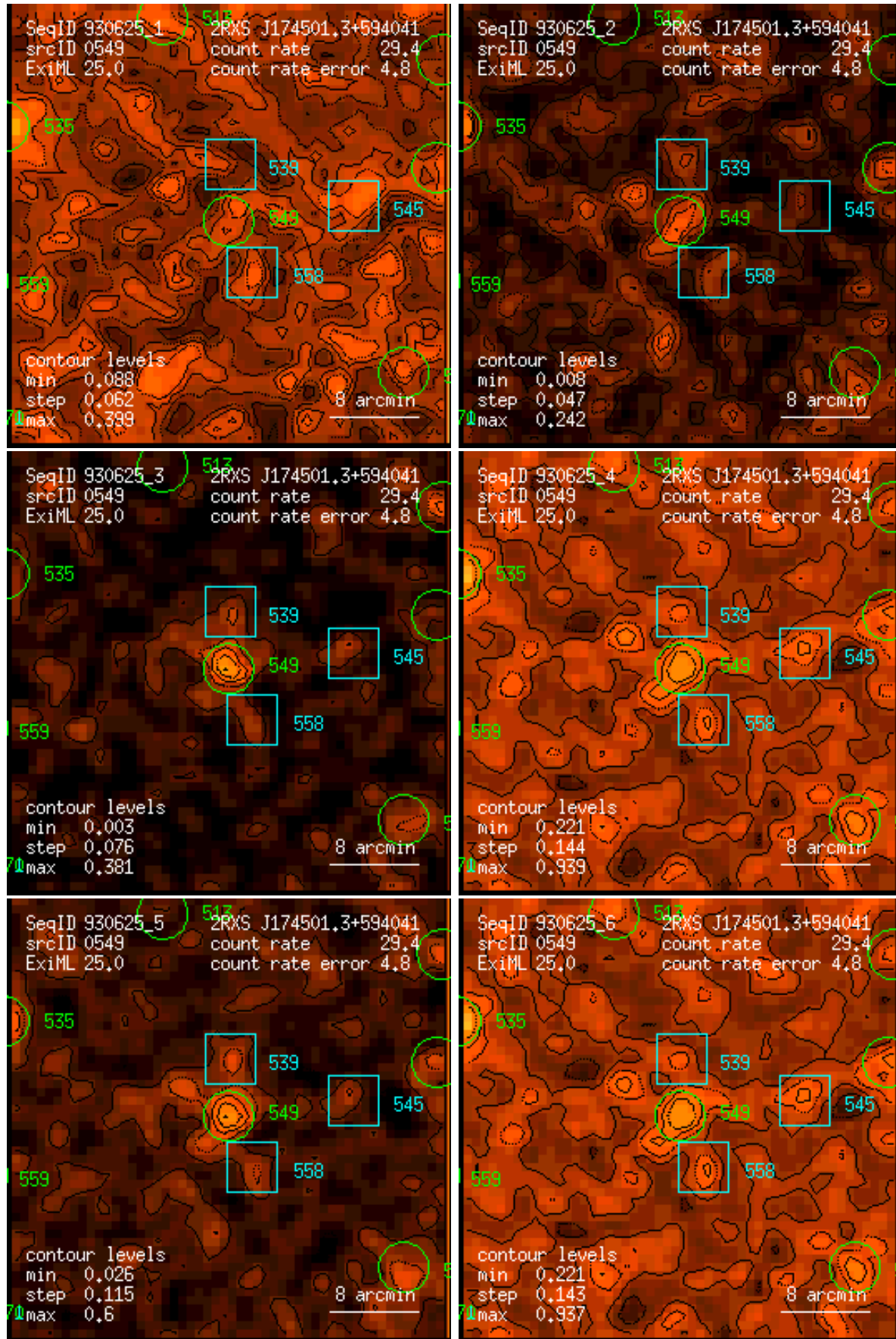
Figure 549: RASS 930625: detection 0549: band rate images, Gaussian filter: (1) PSPC channels 11 – 41, (2) 52 – 90, (3) 91 – 201, (4) 11 – 235, (5) 52 – 201, (6) 11 – 201. Broad band rates in counts/ks. Band rate contour levels in counts/ks/arcmin 2 .
