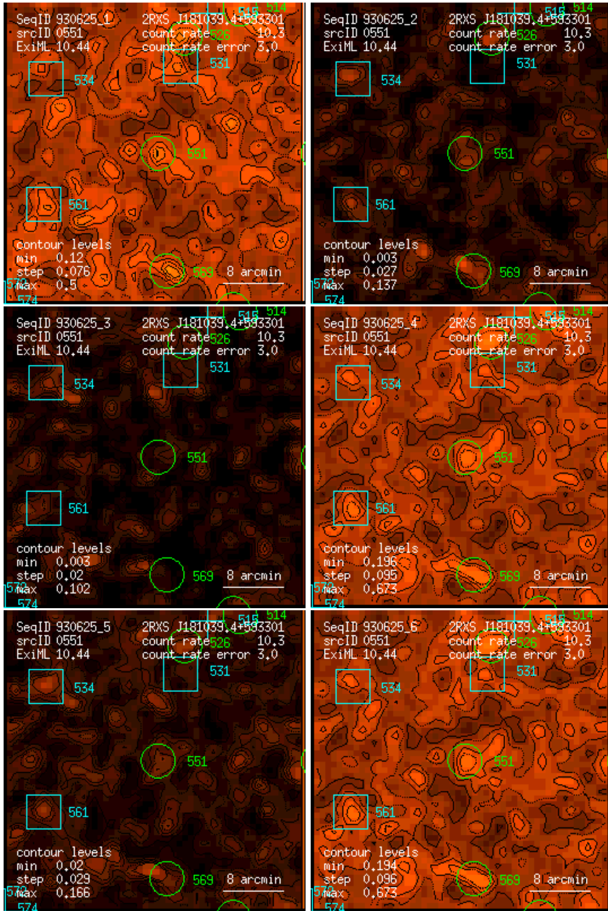
Figure 551: RASS 930625: detection 0551: band rate images, Gaussian filter: (1) PSPC channels 11 – 41, (2) 52 – 90, (3) 91 – 201, (4) 11 – 235, (5) 52 – 201, (6) 11 – 201. Broad band rates in counts/ks. Band rate contour levels in counts/ks/arcmin 2 .
