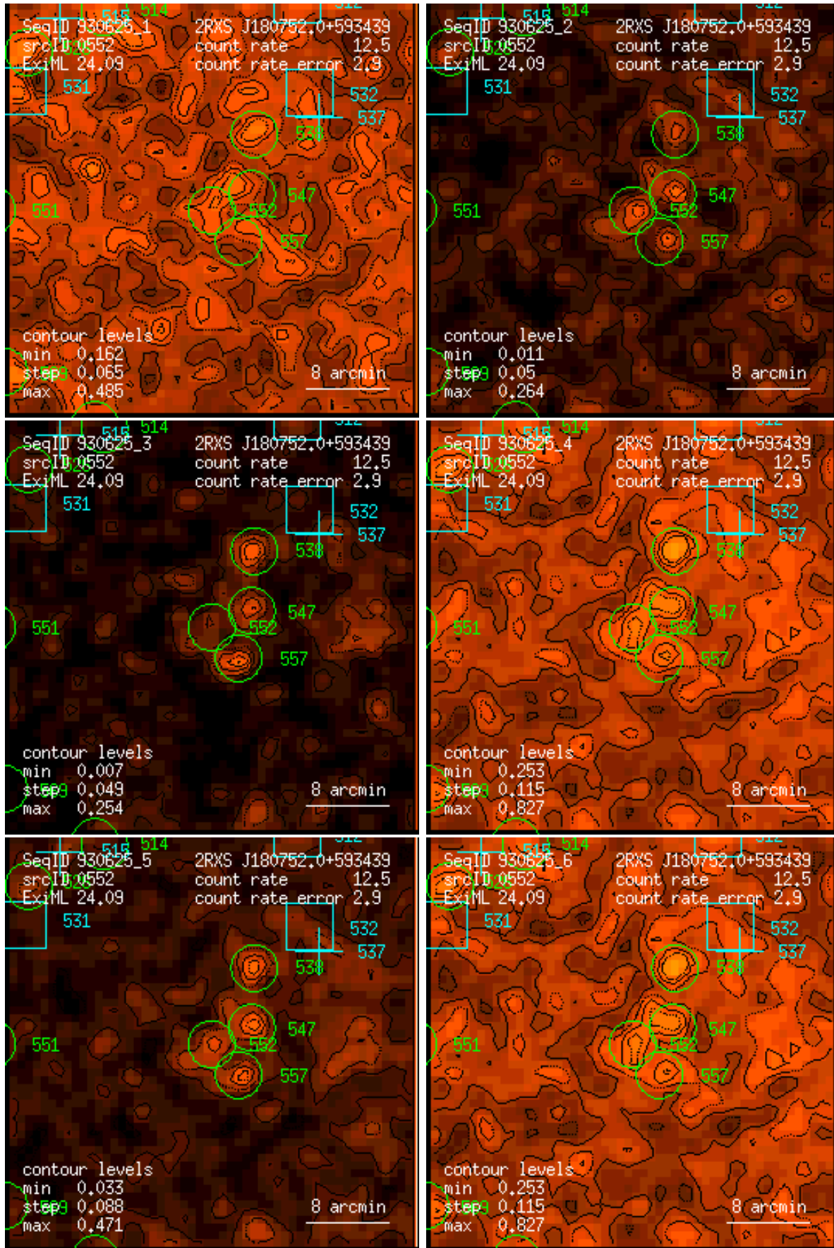
Figure 552: RASS 930625: detection 0552: band rate images, Gaussian filter: (1) PSPC channels 11 – 41, (2) 52 – 90, (3) 91 – 201, (4) 11 – 235, (5) 52 – 201, (6) 11 – 201. Broad band rates in counts/ks. Band rate contour levels in counts/ks/arcmin 2 .
