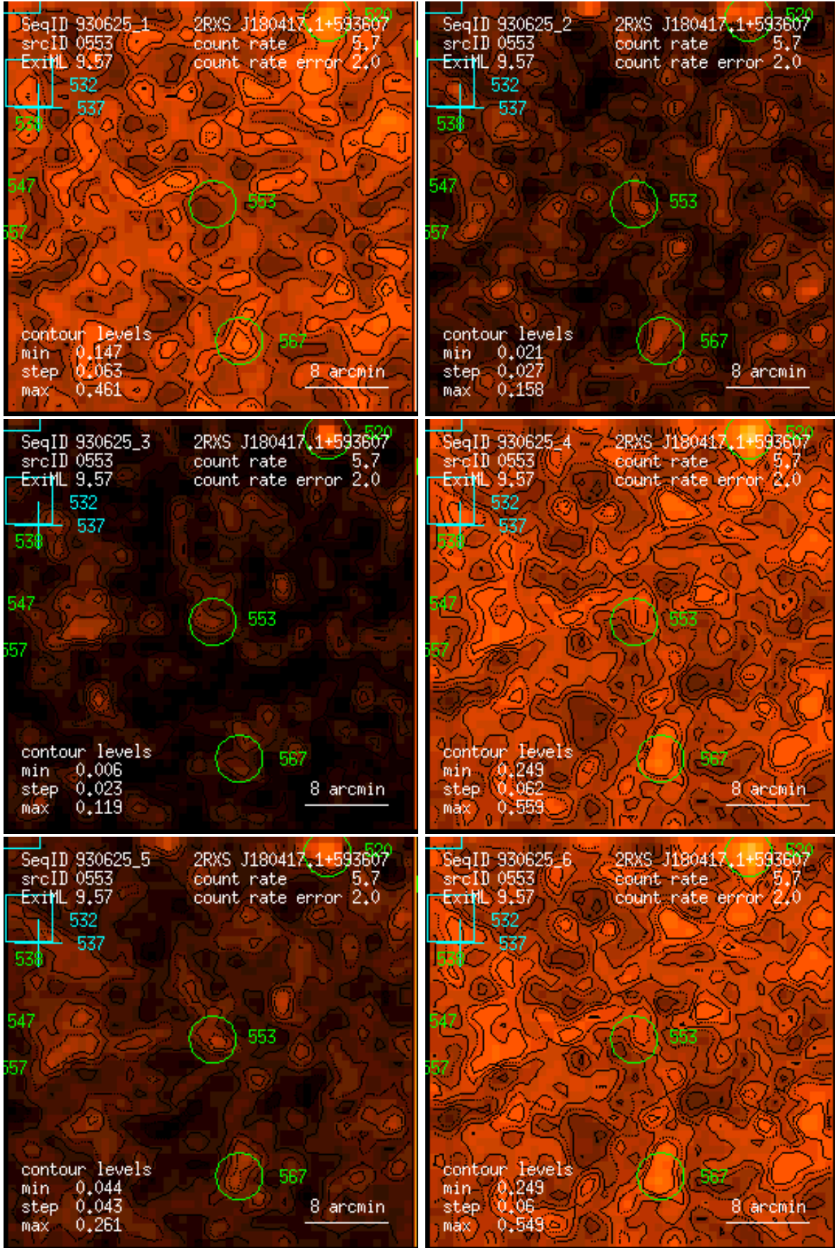
Figure 553: RASS 930625: detection 0553: band rate images, Gaussian filter: (1) PSPC channels 11 – 41, (2) 52 – 90, (3) 91 – 201, (4) 11 – 235, (5) 52 – 201, (6) 11 – 201. Broad band rates in counts/ks. Band rate contour levels in counts/ks/arcmin 2 .
