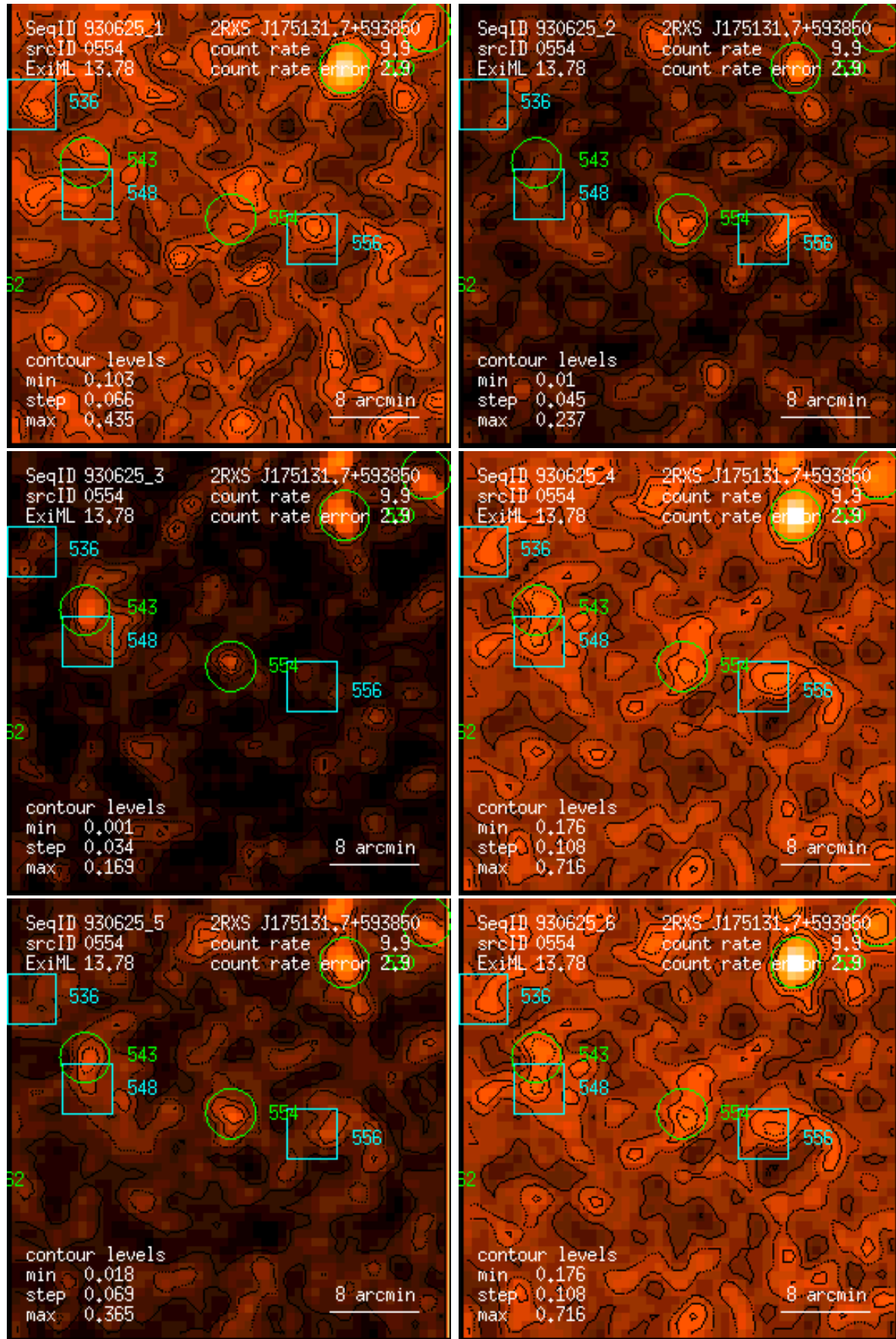
Figure 554: RASS 930625: detection 0554: band rate images, Gaussian filter: (1) PSPC channels 11 – 41, (2) 52 – 90, (3) 91 – 201, (4) 11 – 235, (5) 52 – 201, (6) 11 – 201. Broad band rates in counts/ks. Band rate contour levels in counts/ks/arcmin 2 .
