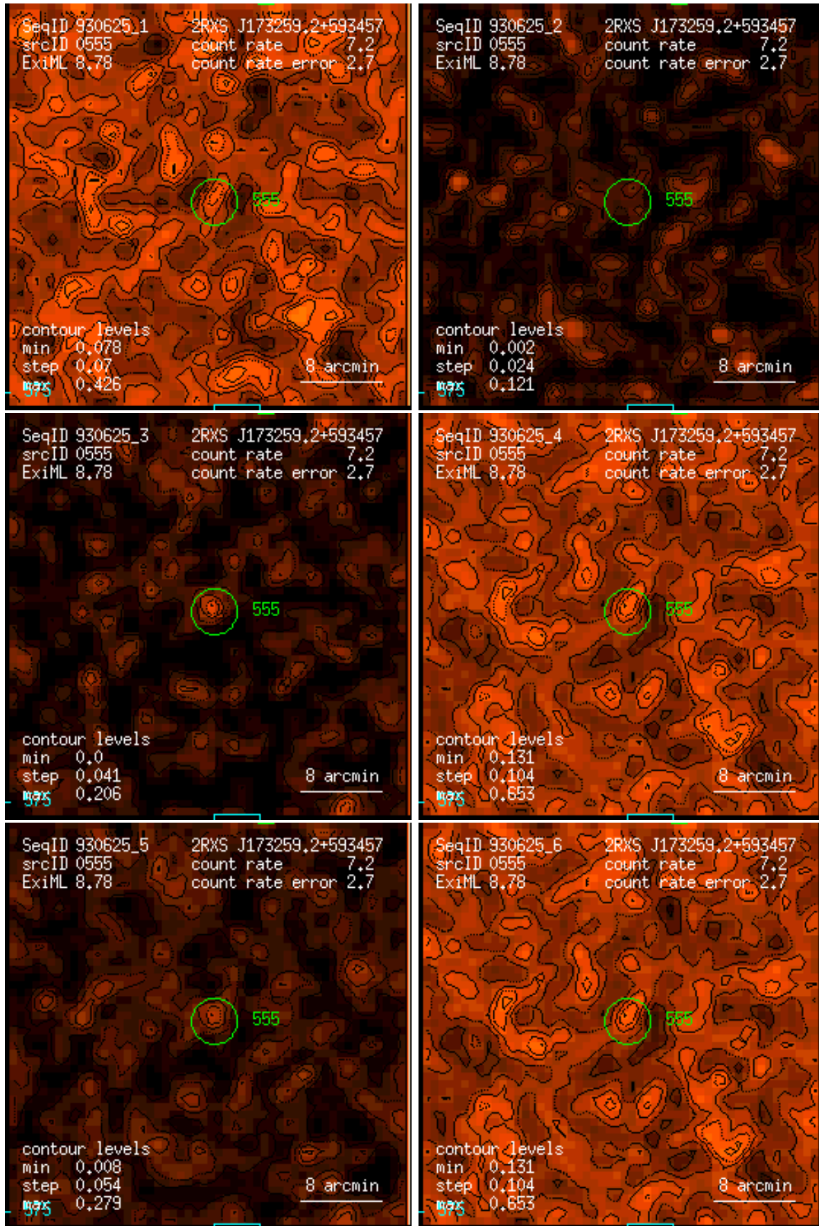
Figure 555: RASS 930625: detection 0555: band rate images, Gaussian filter: (1) PSPC channels 11 – 41, (2) 52 – 90, (3) 91 – 201, (4) 11 – 235, (5) 52 – 201, (6) 11 – 201. Broad band rates in counts/ks. Band rate contour levels in counts/ks/arcmin 2 .
