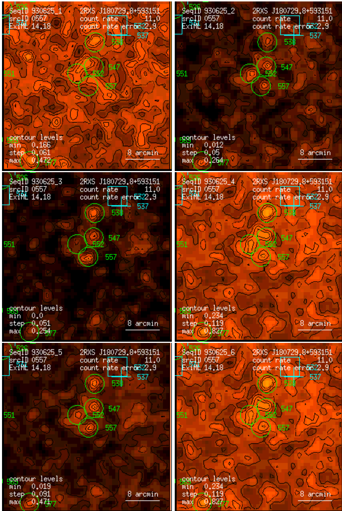
Figure 557: RASS 930625: detection 0557: band rate images, Gaussian filter: (1) PSPC channels 11 – 41, (2) 52 – 90, (3) 91 – 201, (4) 11 – 235, (5) 52 – 201, (6) 11 – 201. Broad band rates in counts/ks. Band rate contour levels in counts/ks/arcmin 2 .
