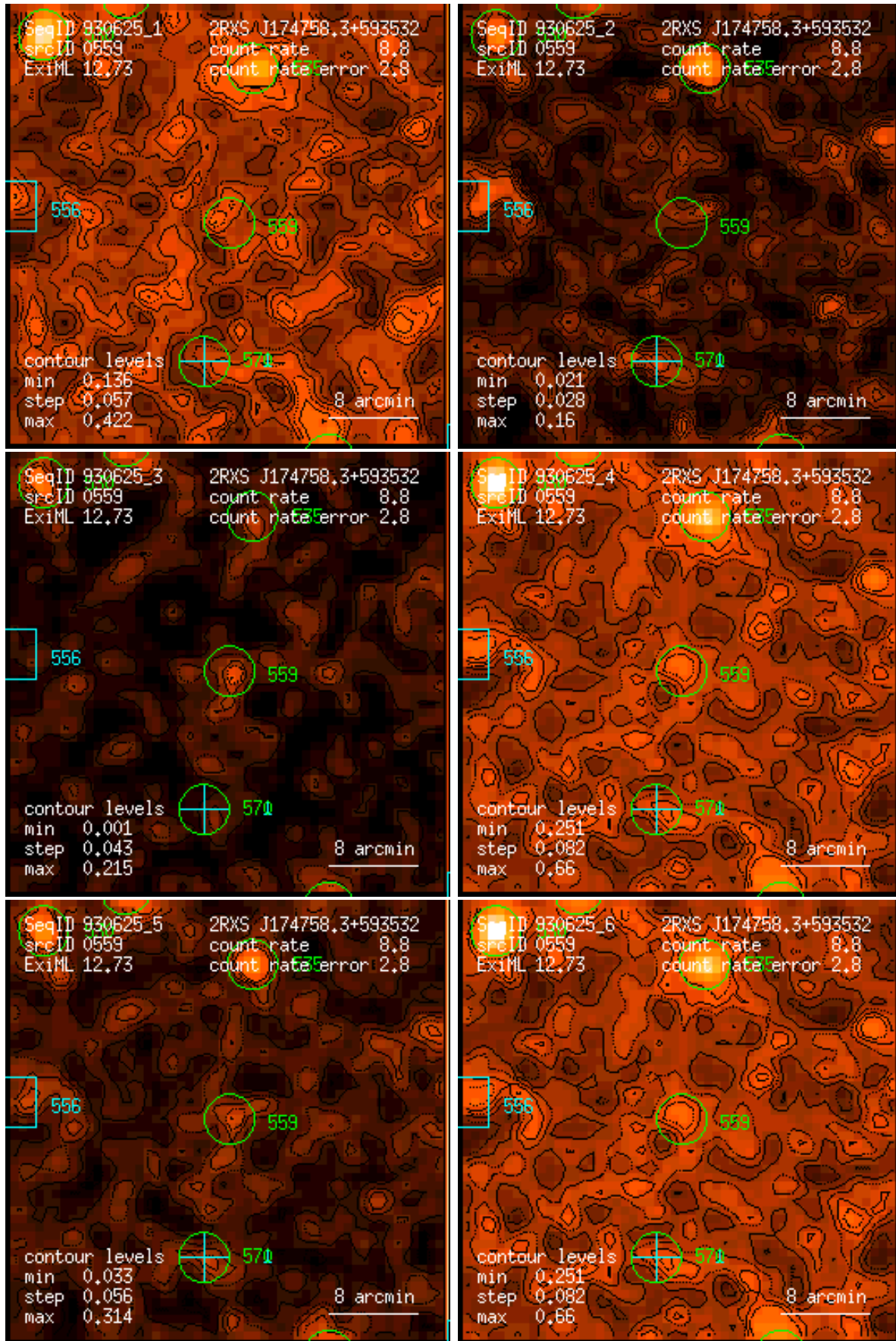
Figure 559: RASS 930625: detection 0559: band rate images, Gaussian filter: (1) PSPC channels 11 – 41, (2) 52 – 90, (3) 91 – 201, (4) 11 – 235, (5) 52 – 201, (6) 11 – 201. Broad band rates in counts/ks. Band rate contour levels in counts/ks/arcmin 2 .
