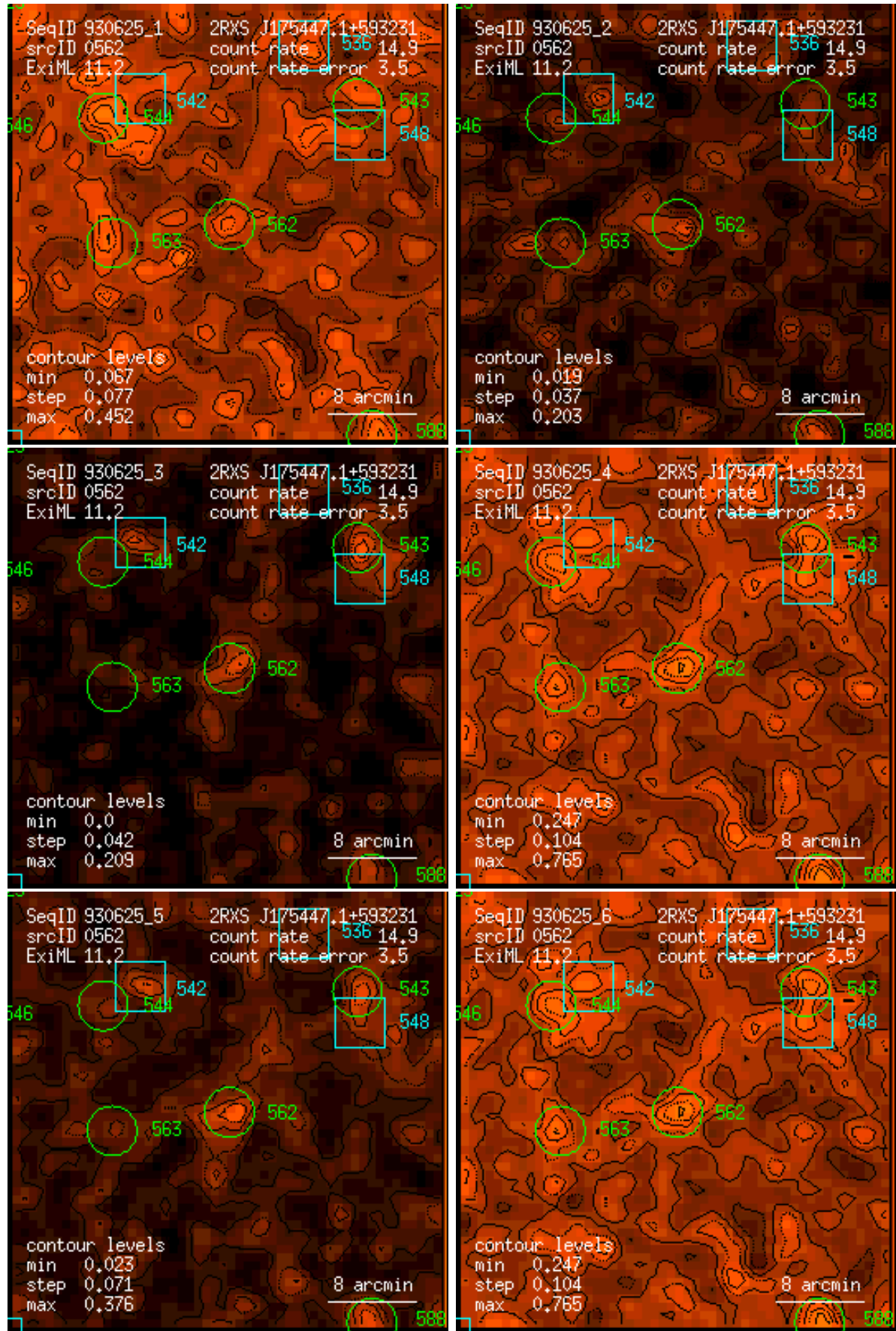
Figure 562: RASS 930625: detection 0562: band rate images, Gaussian filter: (1) PSPC channels 11 – 41, (2) 52 – 90, (3) 91 – 201, (4) 11 – 235, (5) 52 – 201, (6) 11 – 201. Broad band rates in counts/ks. Band rate contour levels in counts/ks/arcmin 2 .
