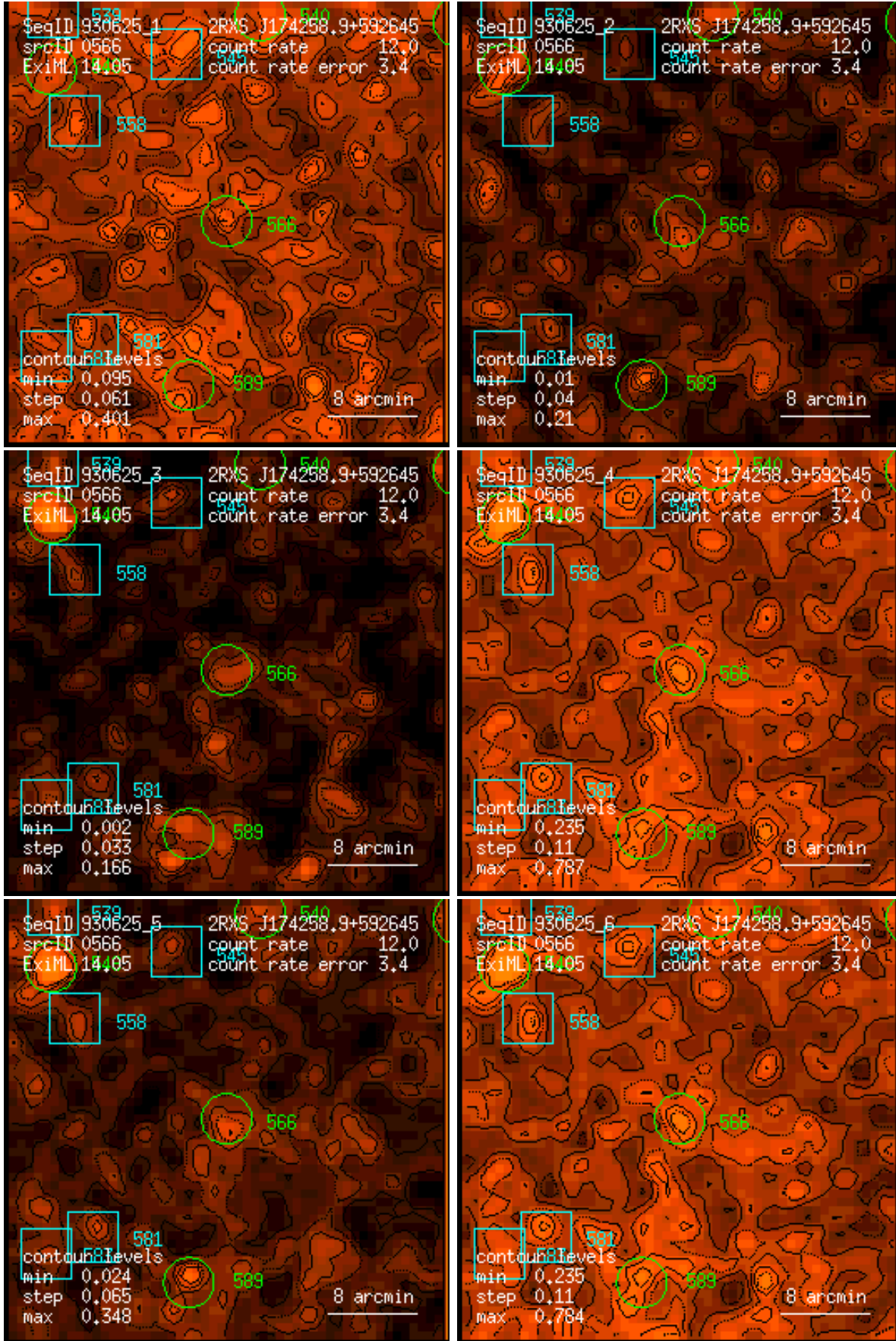
Figure 566: RASS 930625: detection 0566: band rate images, Gaussian filter: (1) PSPC channels 11 – 41, (2) 52 – 90, (3) 91 – 201, (4) 11 – 235, (5) 52 – 201, (6) 11 – 201. Broad band rates in counts/ks. Band rate contour levels in counts/ks/arcmin 2 .
