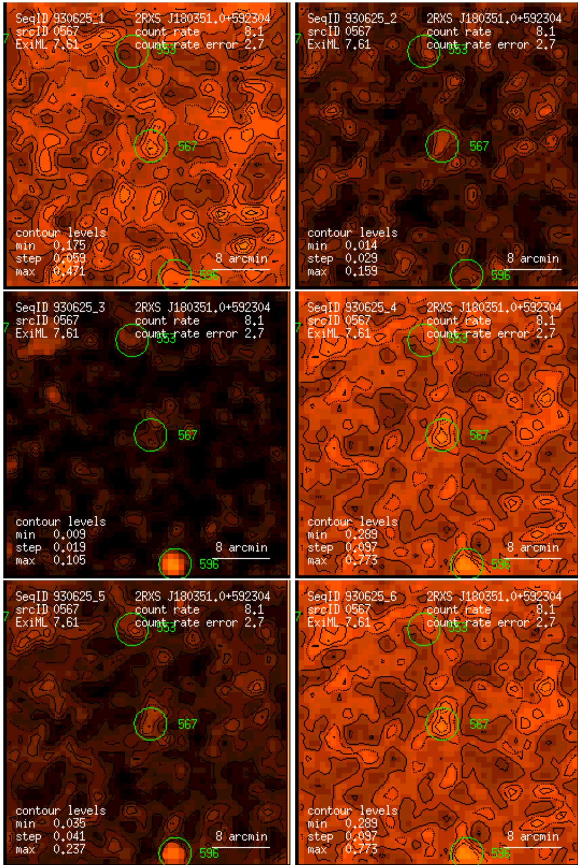
Figure 567: RASS 930625: detection 0567: band rate images, Gaussian filter: (1) PSPC channels 11 – 41, (2) 52 – 90, (3) 91 – 201, (4) 11 – 235, (5) 52 – 201, (6) 11 – 201. Broad band rates in counts/ks. Band rate contour levels in counts/ks/arcmin 2 .
