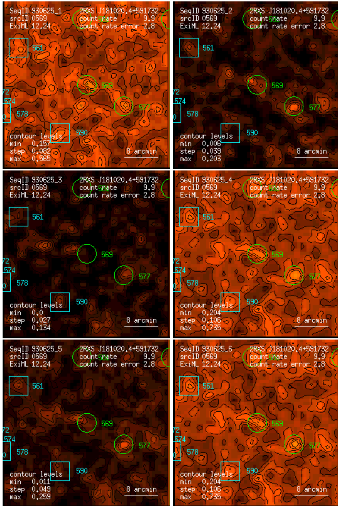
Figure 569: RASS 930625: detection 0569: band rate images, Gaussian filter: (1) PSPC channels 11 – 41, (2) 52 – 90, (3) 91 – 201, (4) 11 – 235, (5) 52 – 201, (6) 11 – 201. Broad band rates in counts/ks. Band rate contour levels in counts/ks/arcmin 2 .
