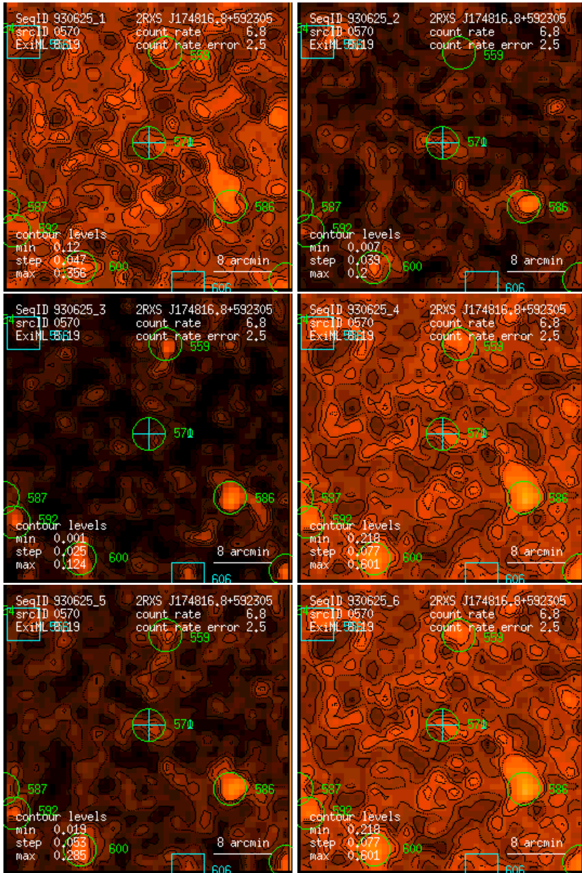
Figure 570: RASS 930625: detection 0570: band rate images, Gaussian filter: (1) PSPC channels 11 – 41, (2) 52 – 90, (3) 91 – 201, (4) 11 – 235, (5) 52 – 201, (6) 11 – 201. Broad band rates in counts/ks. Band rate contour levels in counts/ks/arcmin 2 .
