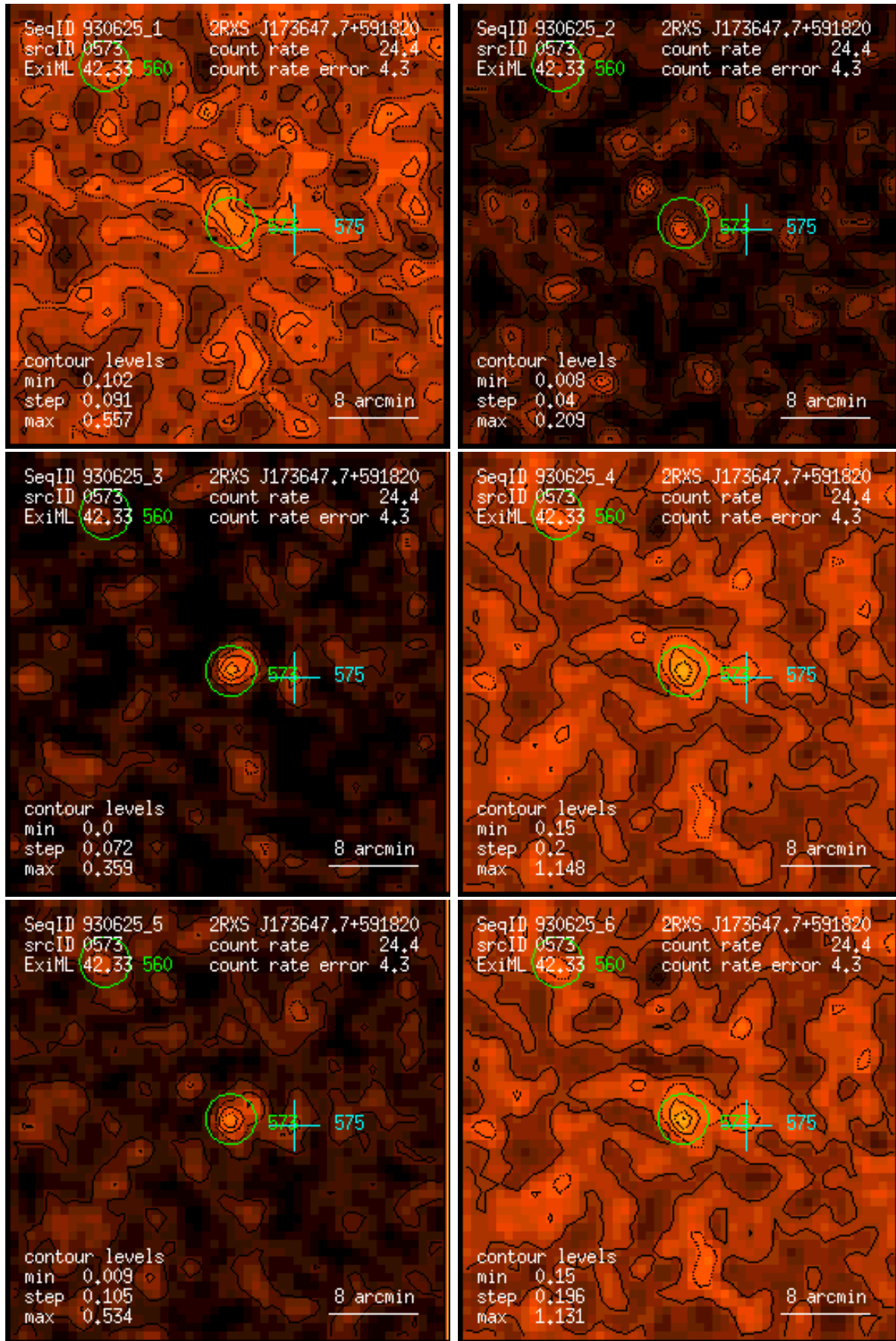
Figure 573: RASS 930625: detection 0573: band rate images, Gaussian filter: (1) PSPC channels 11 – 41, (2) 52 – 90, (3) 91 – 201, (4) 11 – 235, (5) 52 – 201, (6) 11 – 201. Broad band rates in counts/ks. Band rate contour levels in counts/ks/arcmin 2 .
