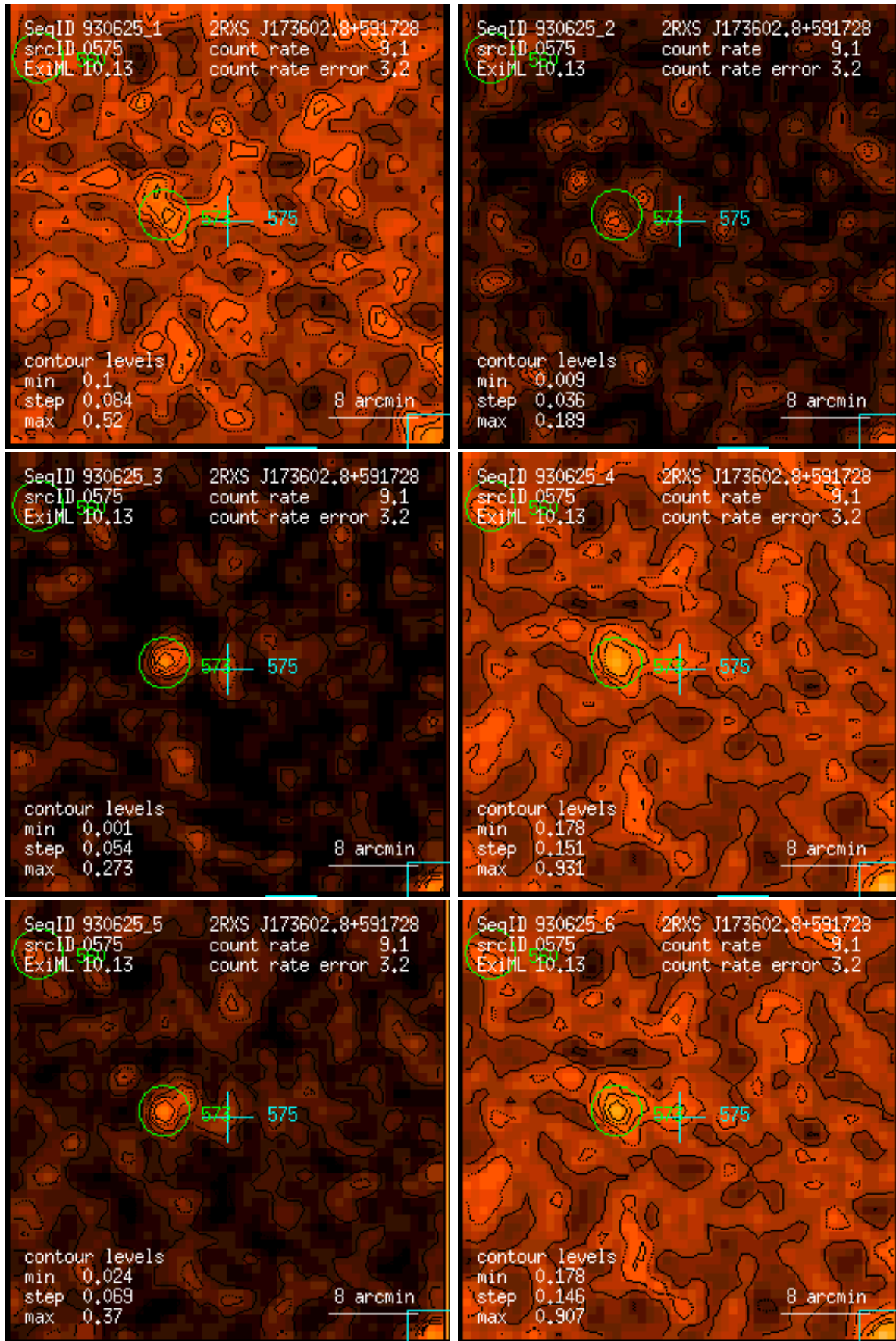
Figure 575: RASS 930625: detection 0575: band rate images, Gaussian filter: (1) PSPC channels 11 – 41, (2) 52 – 90, (3) 91 – 201, (4) 11 – 235, (5) 52 – 201, (6) 11 – 201. Broad band rates in counts/ks. Band rate contour levels in counts/ks/arcmin 2 .
