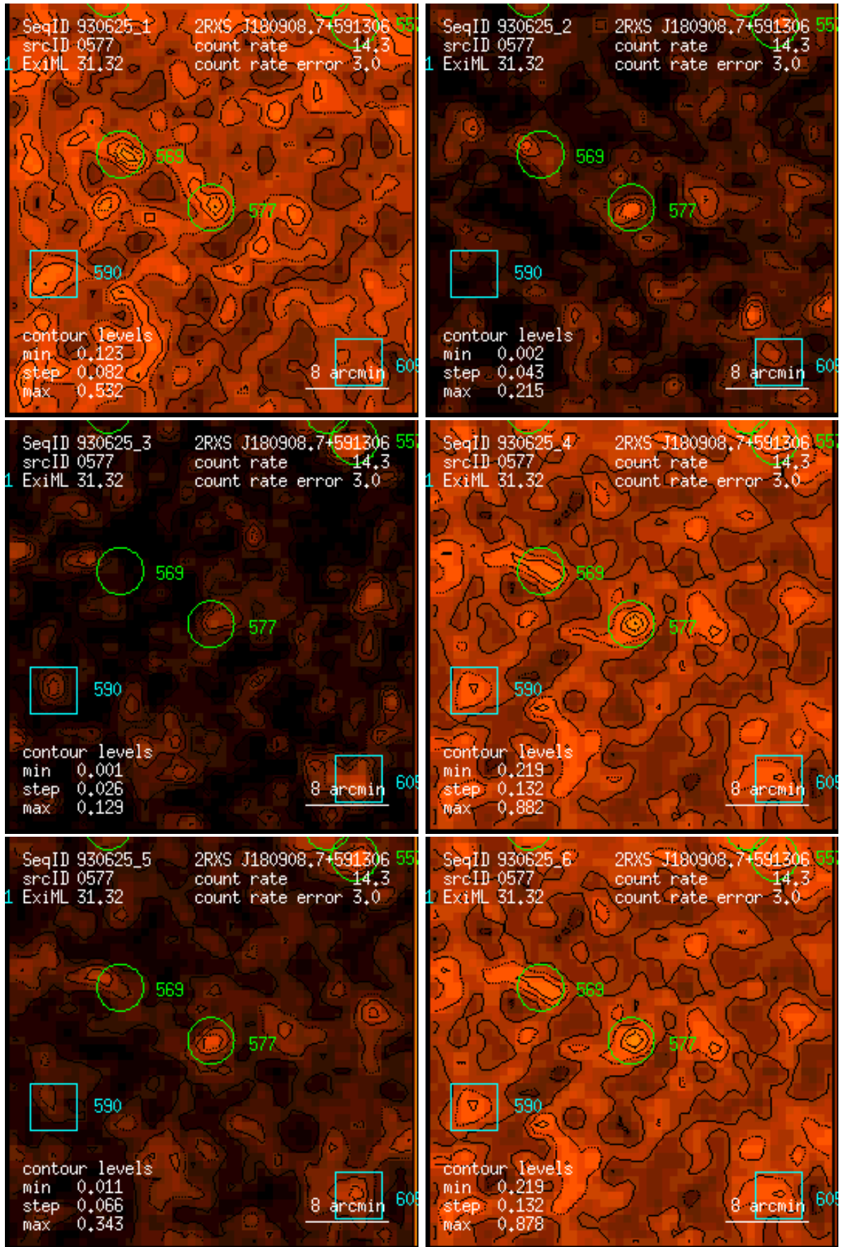
Figure 577: RASS 930625: detection 0577: band rate images, Gaussian filter: (1) PSPC channels 11 – 41, (2) 52 – 90, (3) 91 – 201, (4) 11 – 235, (5) 52 – 201, (6) 11 – 201. Broad band rates in counts/ks. Band rate contour levels in counts/ks/arcmin 2 .
