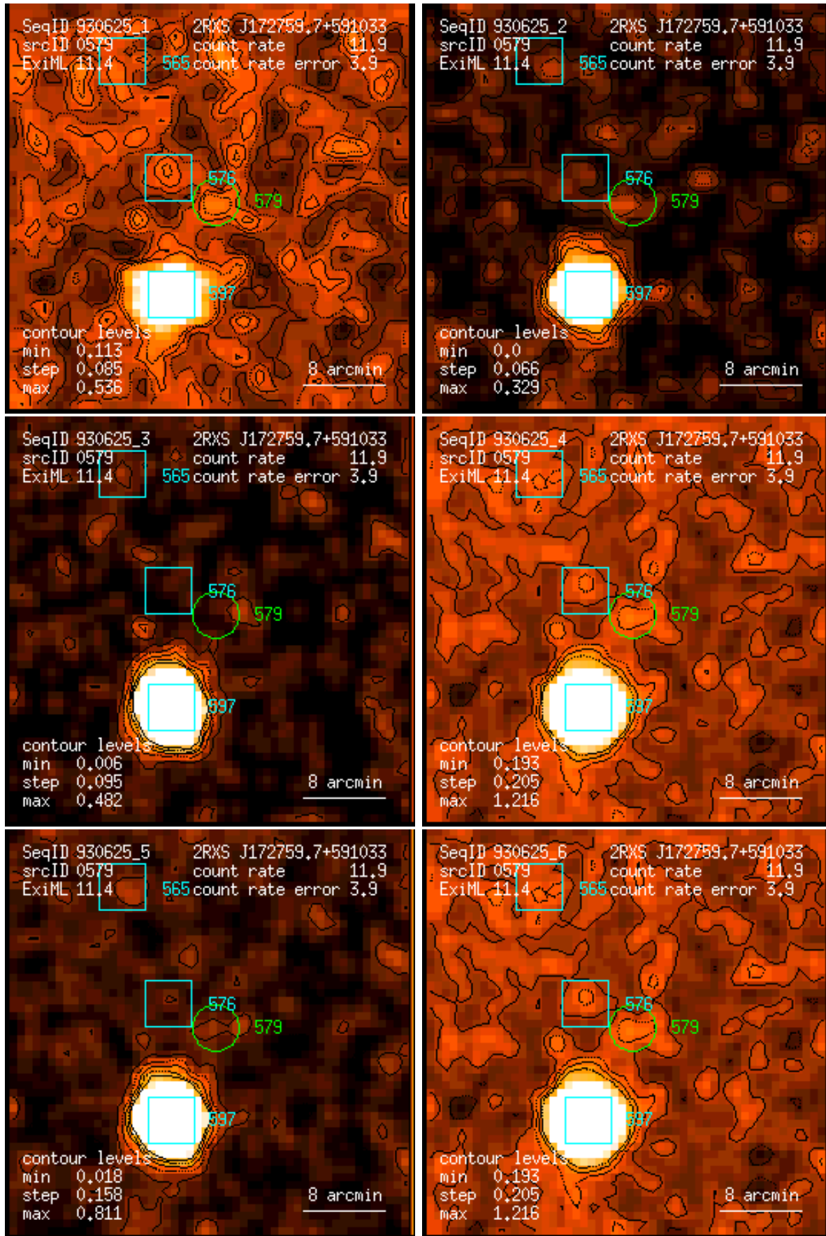
Figure 579: RASS 930625: detection 0579: band rate images, Gaussian filter: (1) PSPC channels 11 – 41, (2) 52 – 90, (3) 91 – 201, (4) 11 – 235, (5) 52 – 201, (6) 11 – 201. Broad band rates in counts/ks. Band rate contour levels in counts/ks/arcmin 2 .
