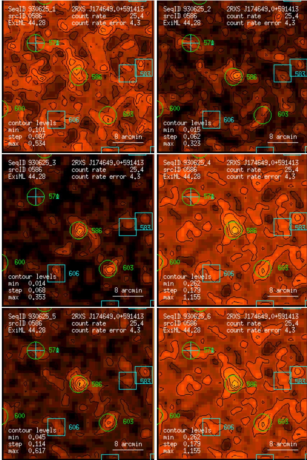
Figure 586: RASS 930625: detection 0586: band rate images, Gaussian filter: (1) PSPC channels 11 – 41, (2) 52 – 90, (3) 91 – 201, (4) 11 – 235, (5) 52 – 201, (6) 11 – 201. Broad band rates in counts/ks. Band rate contour levels in counts/ks/arcmin 2 .
