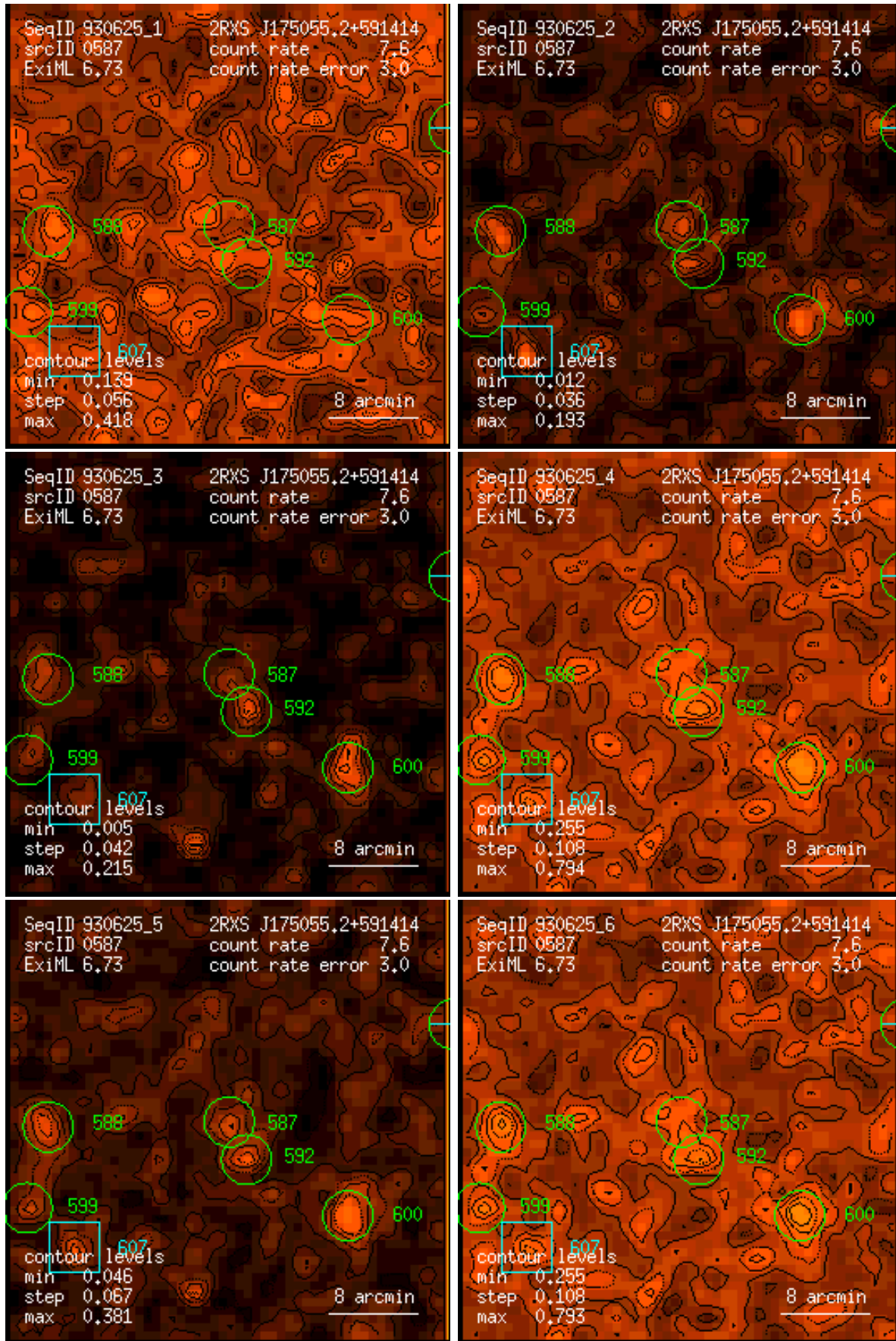
Figure 587: RASS 930625: detection 0587: band rate images, Gaussian filter: (1) PSPC channels 11 – 41, (2) 52 – 90, (3) 91 – 201, (4) 11 – 235, (5) 52 – 201, (6) 11 – 201. Broad band rates in counts/ks. Band rate contour levels in counts/ks/arcmin 2 .
