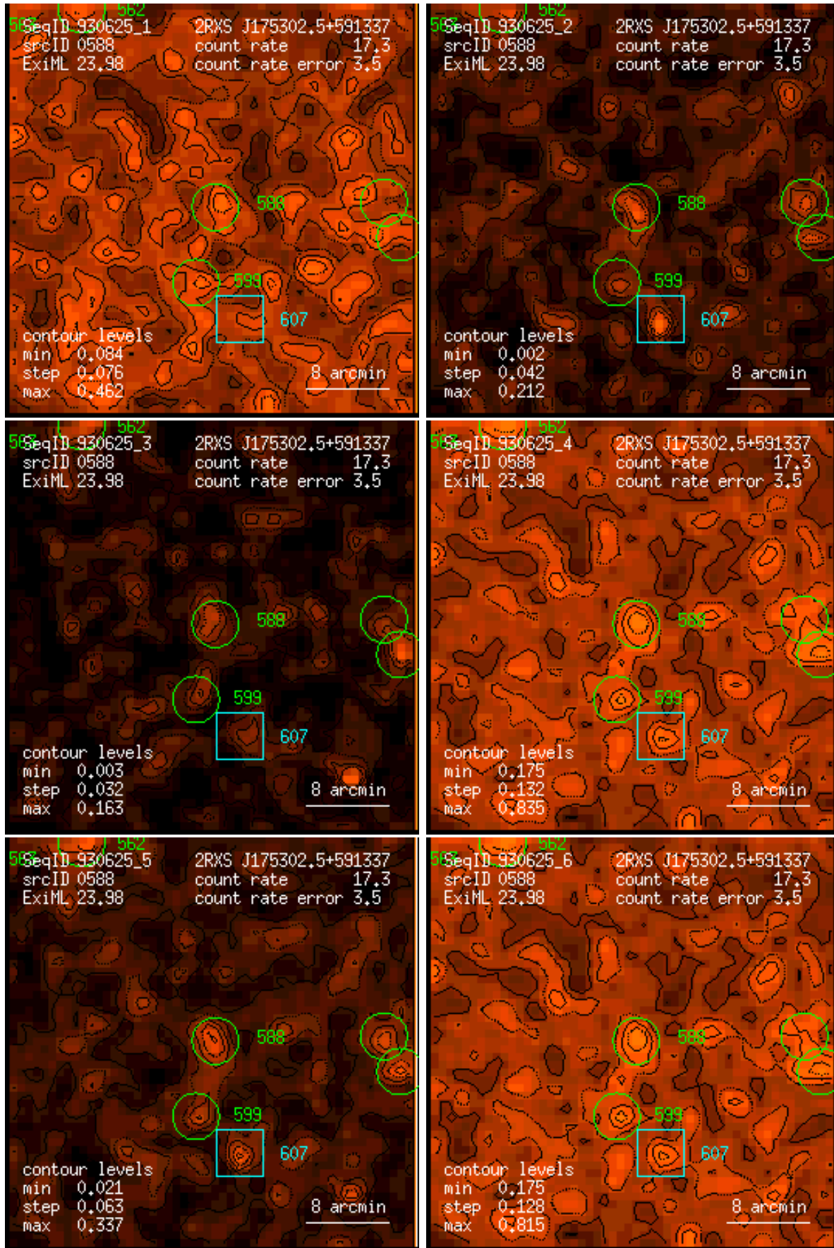
Figure 588: RASS 930625: detection 0588: band rate images, Gaussian filter: (1) PSPC channels 11 – 41, (2) 52 – 90, (3) 91 – 201, (4) 11 – 235, (5) 52 – 201, (6) 11 – 201. Broad band rates in counts/ks. Band rate contour levels in counts/ks/arcmin 2 .
