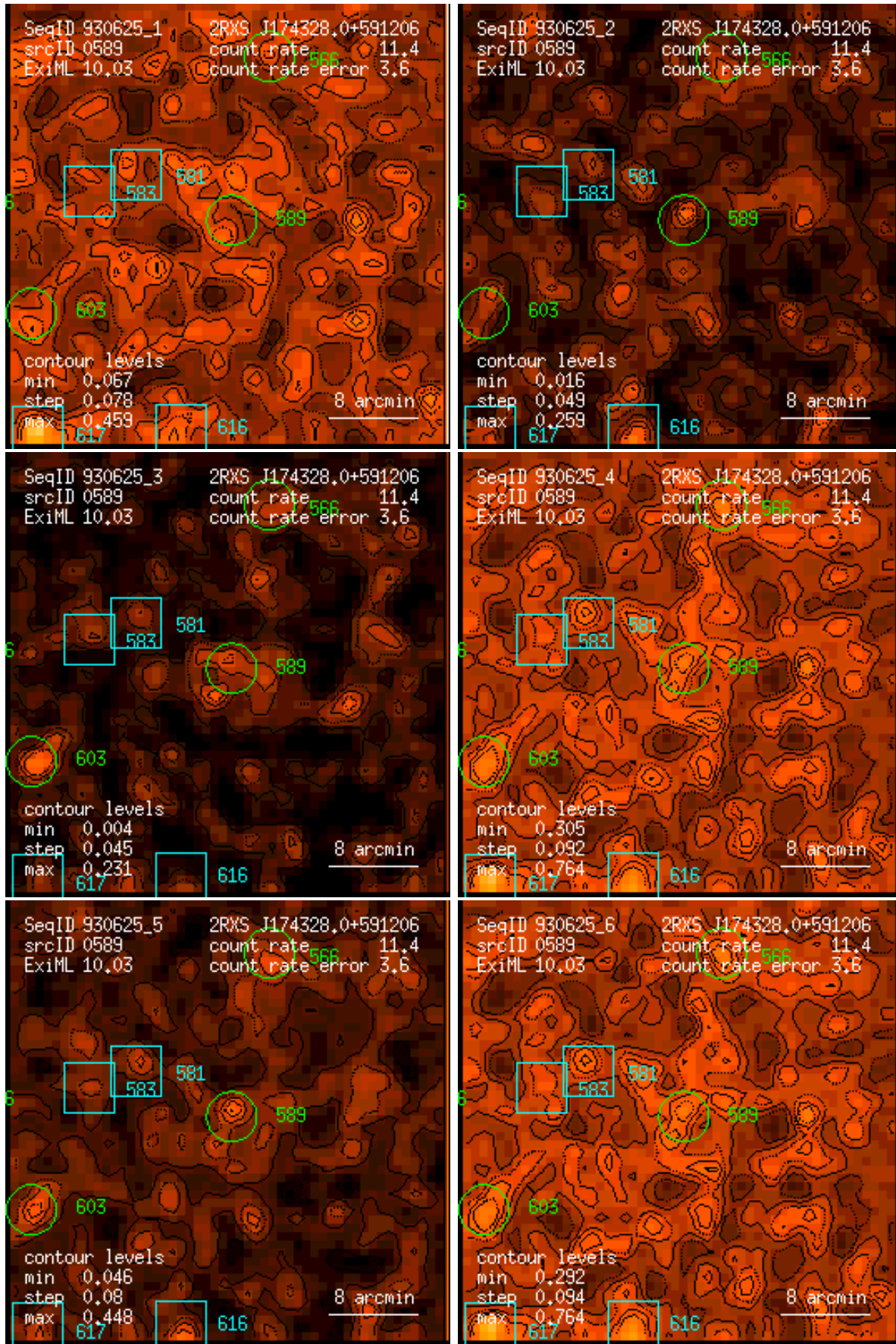
Figure 589: RASS 930625: detection 0589: band rate images, Gaussian filter: (1) PSPC channels 11 – 41, (2) 52 – 90, (3) 91 – 201, (4) 11 – 235, (5) 52 – 201, (6) 11 – 201. Broad band rates in counts/ks. Band rate contour levels in counts/ks/arcmin 2 .
