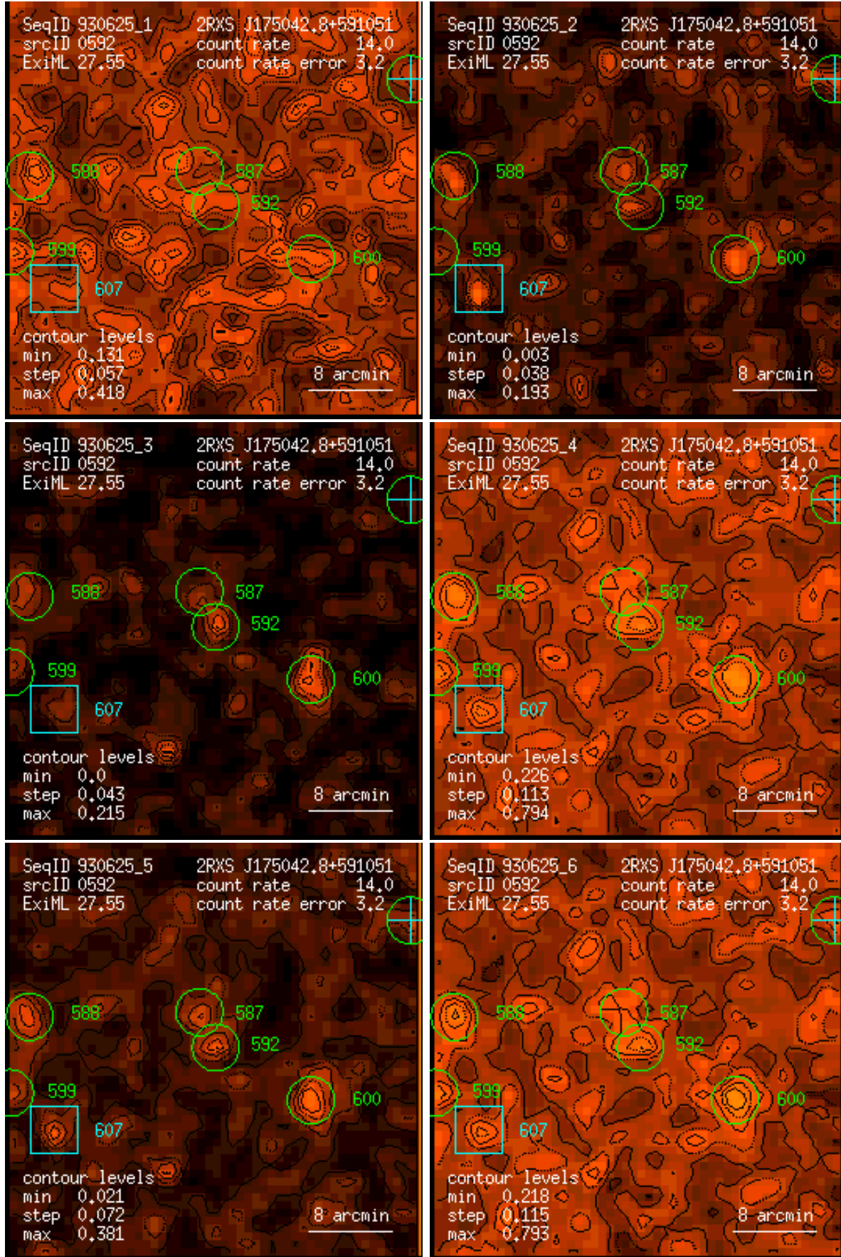
Figure 592: RASS 930625: detection 0592: band rate images, Gaussian filter: (1) PSPC channels 11 – 41, (2) 52 – 90, (3) 91 – 201, (4) 11 – 235, (5) 52 – 201, (6) 11 – 201. Broad band rates in counts/ks. Band rate contour levels in counts/ks/arcmin 2 .
